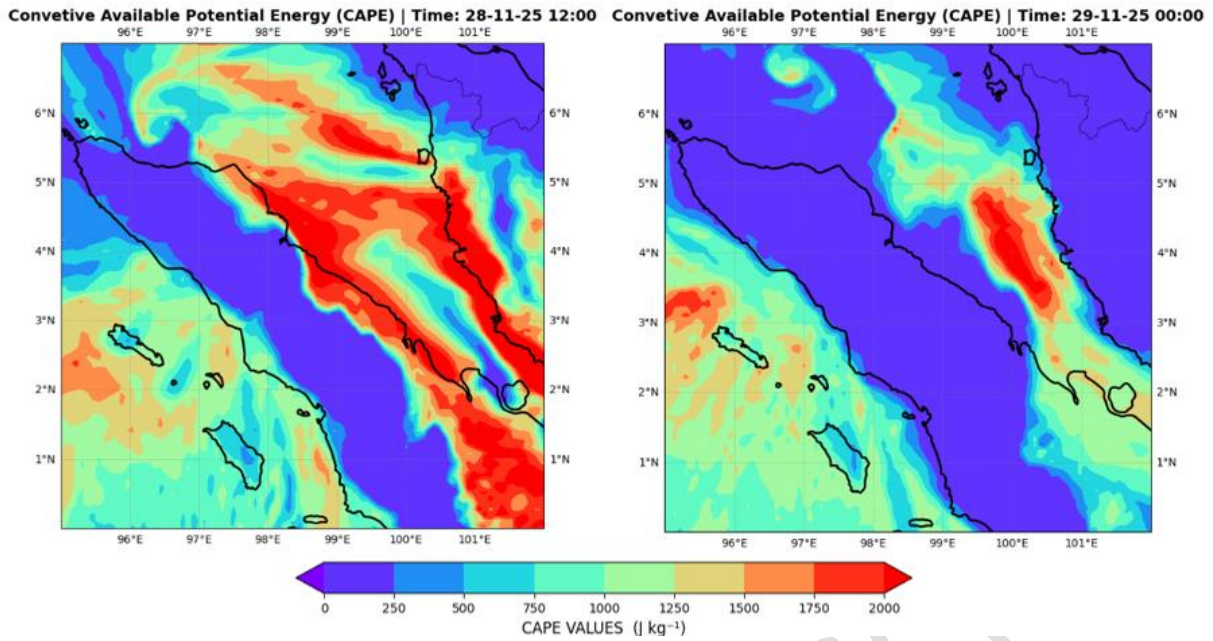
Figure 21. CAPE ( \text{J kg}^{-1} ) on 28–29 November 2025 during dissipation.
