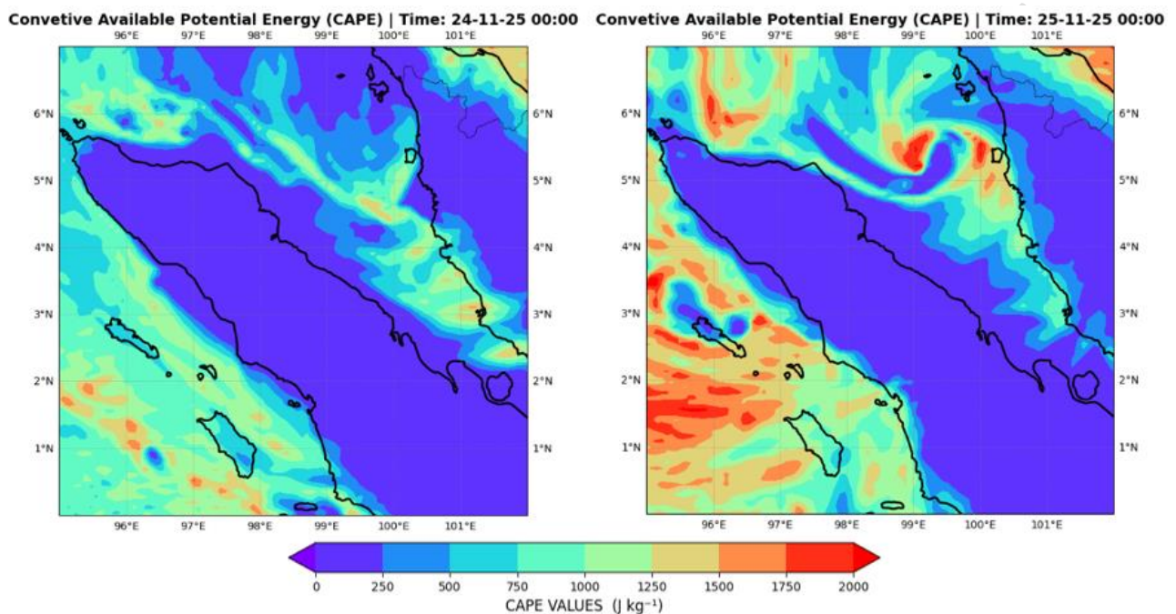
Figure 4. CAPE (J kg -1 ) on 24–25 November 2025 showing increasing convective instability prior to cyclogenesis.
