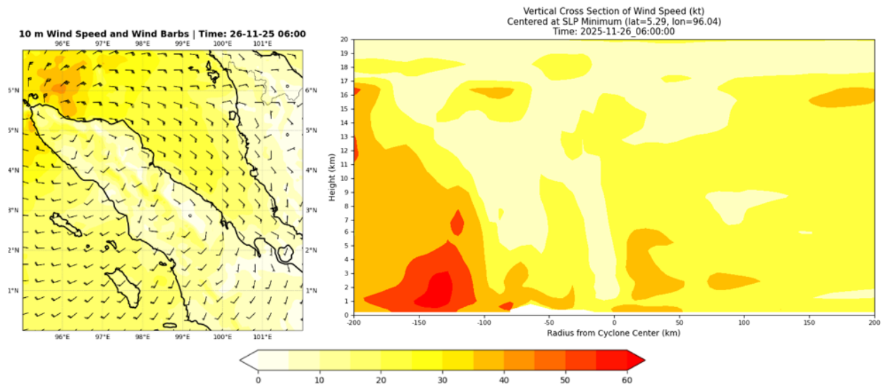
Figure 18. Horizontal wind speed and streamlines at 850 hPa on 26 Nov 2025 at 06 UTC.
