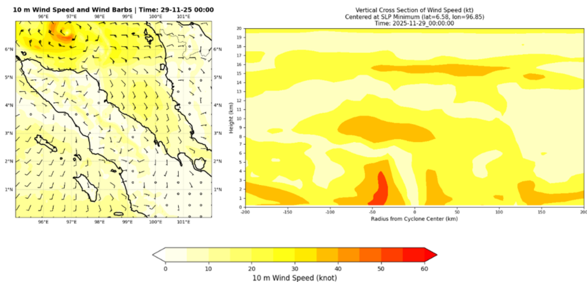
Figure 24. Vertical wind shear 850 - 200 hPa on 29 Nov 2025 at 00 UTC
