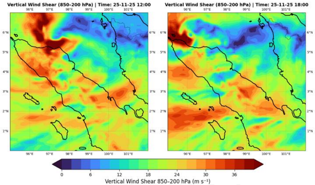
Figure 12. Vertical wind shear (200–850 hPa) on 25 November 2025 at 12 and 18 UTC.
