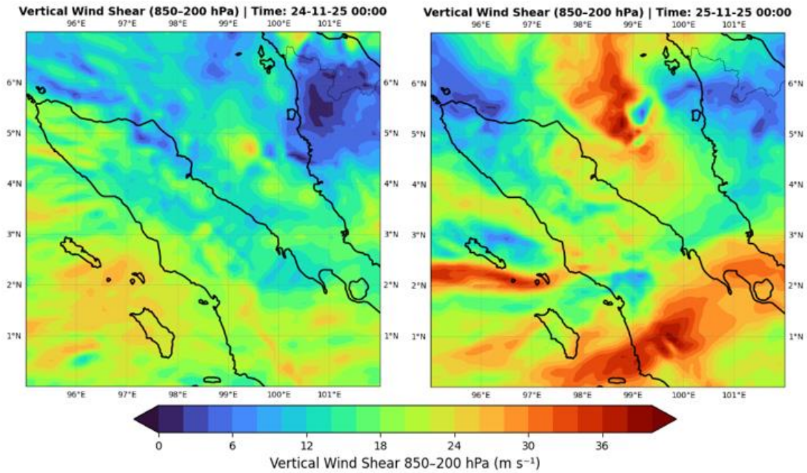
Figure 7. Vertical wind shear (200–850 hPa, \text{m s}^{-1} ) on 24–25 November 2025.
