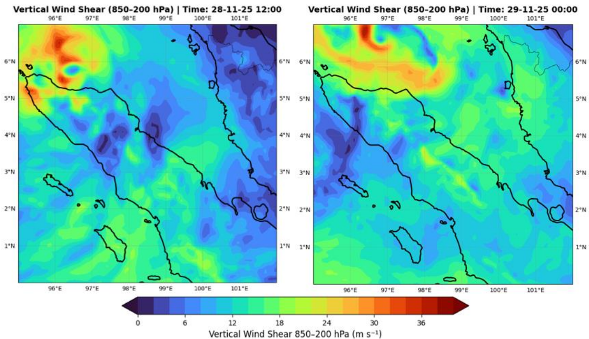
Figure 22. Vertical wind shear on 28–29 November 2025 (dissipation).
