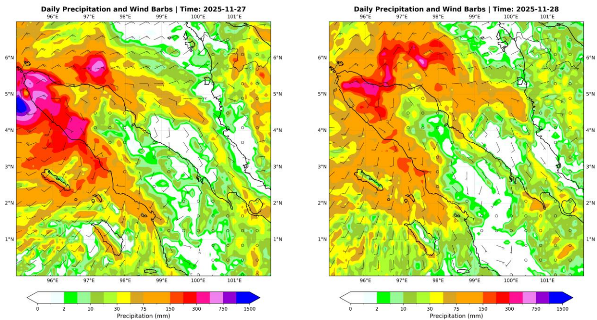
Figure 25. Daily precipitation ( \text{mm day}^{-1} ) and 850-hPa wind barbs from 25 to 28 November 2025.
