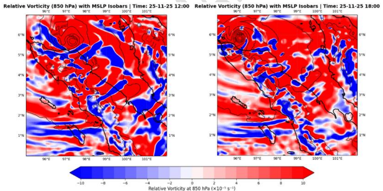
Figure 9. Relative Vorticity with Mean Sea Level Pressure on 25 Nov 2025 at 12 and 18 UTC.
