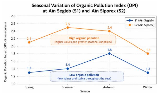
Figure 2. Seasonal variation of of the Organic Pollution Index (OPI) at Ain Segleb (S1) and Ain Siporex (S2). S1 shows low and stable organic pollution throughout the year, whereas S2 exhibits higher values and greater seasonal variability, particularly in summer and autumn.
