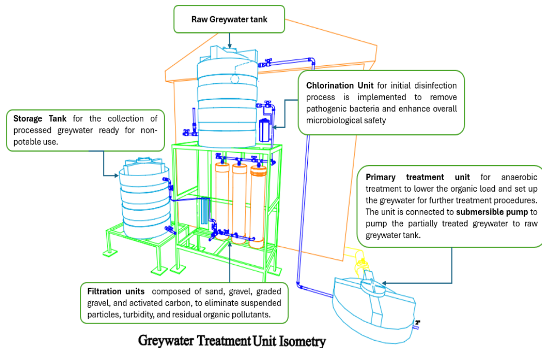
Figure 2 Illustration of the on-site GWTU (CMWU, 2021)
