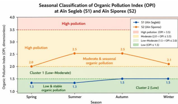
Figure 3. Seasonal classification of the organic pollution index (OPI) at Ain Segleb (S1) and Ain Siporex (S2). OPI values are grouped into four quality classes: High pollution (OPI > 3.5), Moderate (2.0 < OPI ≤ 3.5), Low-Moderate (1.5 < OPI ≤ 2.0), and Low (OPI ≤ 1.5). S1 shows low and stable organic pollution, whereas S2 exhibits moderate and seasonal organic pollution.
