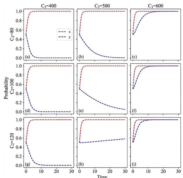
Figure 4. Influence of penalties and subsidies on the strategy evolution of the two participants.
