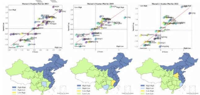
Figure 6. Moran Scatter Plot for 30 provincial regions.
