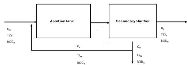
Figure 3. Mass balances in the activated sludge process.
