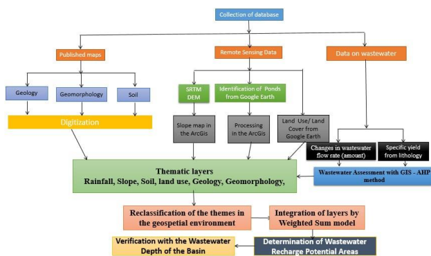
Figure 6. Schematic flow of the study area using GIS and AHP methods.
