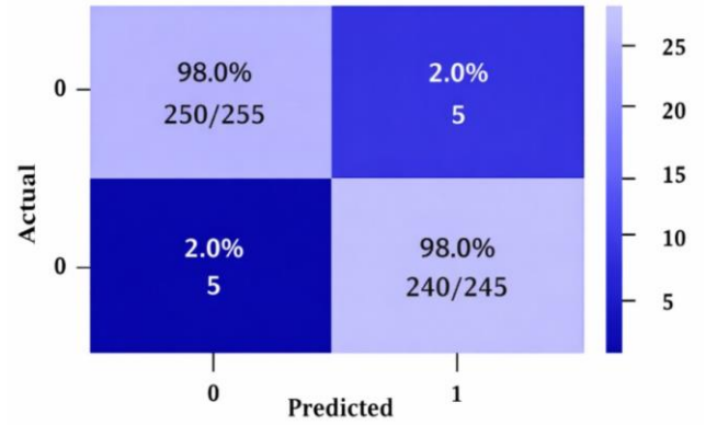
Figure 5. Confusion matrix
