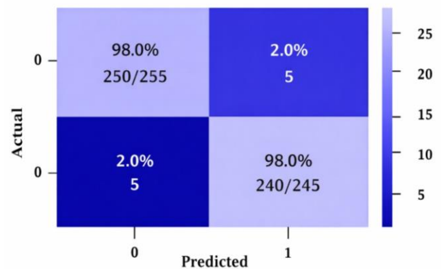
Figure 5. Confusion matrix
