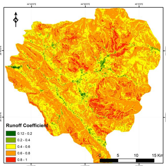
Figure 5. Runoff coefficient (RC) in the basin.
