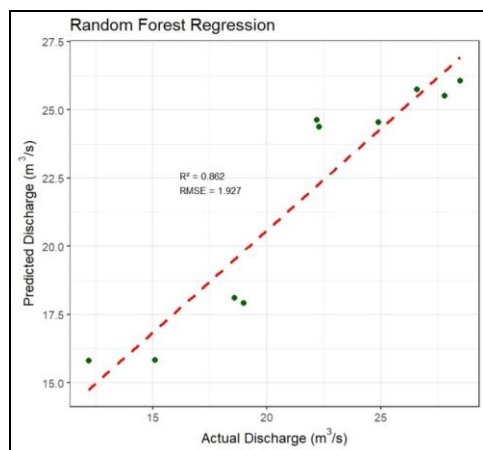
Figure 8. Model Evaluations for Jundian watershed.
