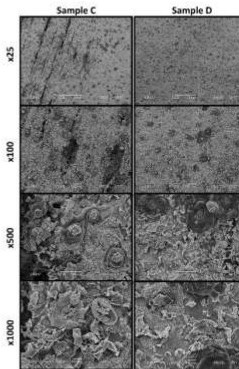
Figure 3b. Micrographs of Samples C and D after immersion in artificial seawater for 10 days
