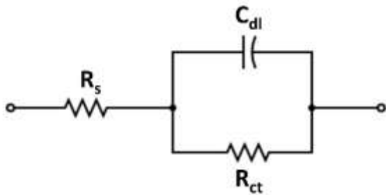
Figure 2. The equivalent electrical circuit (EEC) used to fit EIS data
