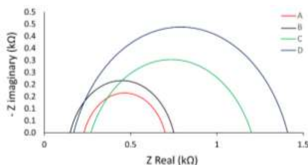
Figure 1. Nyquist curves of mild steel samples after ten days of immersion for samples A – D.
