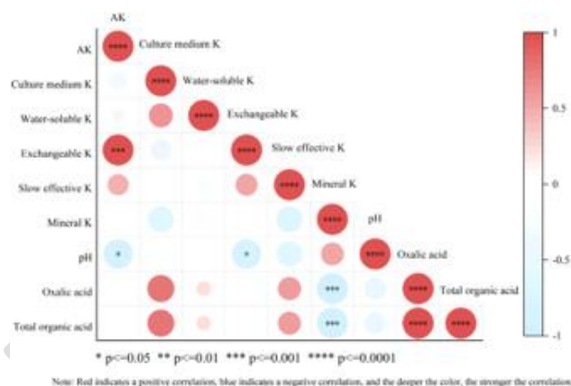
Figure 5. Correlation coefficients of soil potassium cycling factors
