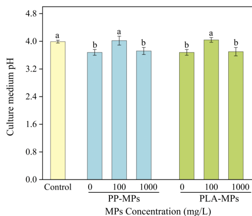
Figure 3. Effect of different types of MPs on the pH of the culture solution. Note: Duncan's post hoc test revealed that different lowercase letters indicated significant differences among the various treatment groups ( P < 0.05 ).
