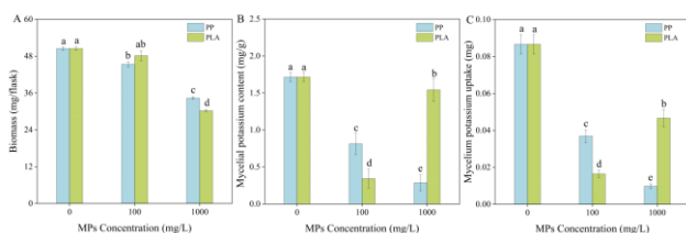
Figure 2. Effects of two MPs on Ld biomass (A), potassium content (B), and potassium uptake (C). Note: Duncan's post hoc test showed that different lowercase letters indicate significant differences ( P < 0.05 ).
