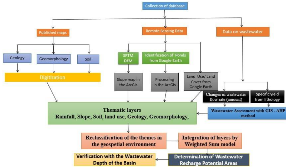
Figure 6. Schematic flow of the study area using GIS and AHP methods
