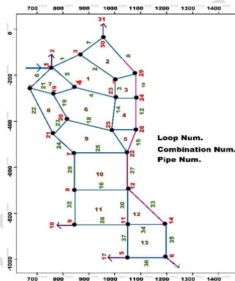
Figure 3. Closed eyes network diagram (Kocaman, 2022)
