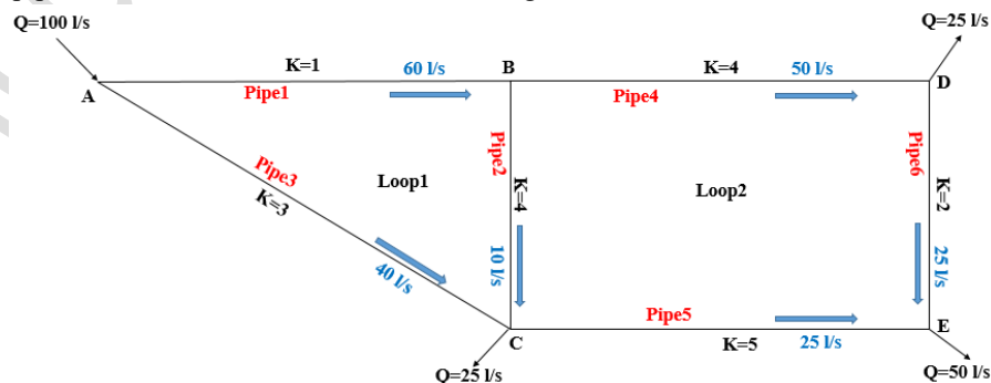
Figure 7. Two-Eye Network
