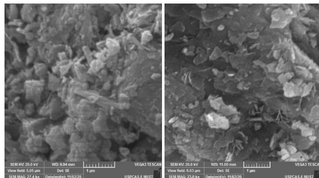
Figure 2. SEM images of pure (a) and \text{TiO}_2 doped \text{ZrO}_2 - \text{SnO}_2 NC (b)
