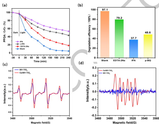
Figure 5. (a) PFOA curve for photocatalytic degradation of Ce/001-TiO 2 for 240min under conditions of capture agent available for different active species. (b) Bar chart depicting the photocatalytic degradation of PFOA by Ce/001-TiO 2 for 240min under conditions of capture agent available for different active species. (c) DMPO- \cdot\text{OH} EPR signal, (d) DMPO- \cdot\text{O}_2^- EPR signal
