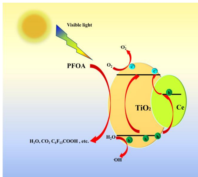
Figure 6. Schematic Illustration of Photocatalytic Degradation of PFOA
