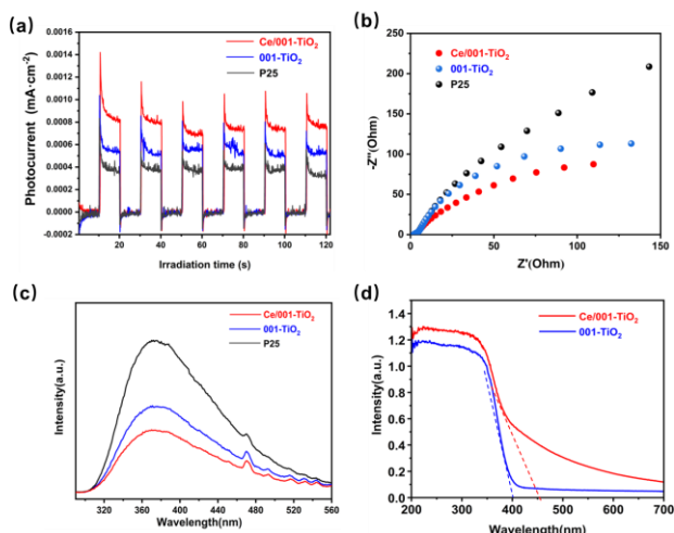
Figure 3. (a) Transient photocurrent response plots ( I-t curves), (b) Electrochemical impedance spectra, (c) Steady-state photoluminescence (PL) spectra, (d) Ultraviolet-visible diffuse reflectance spectroscopy (UV-Vis DRS)
