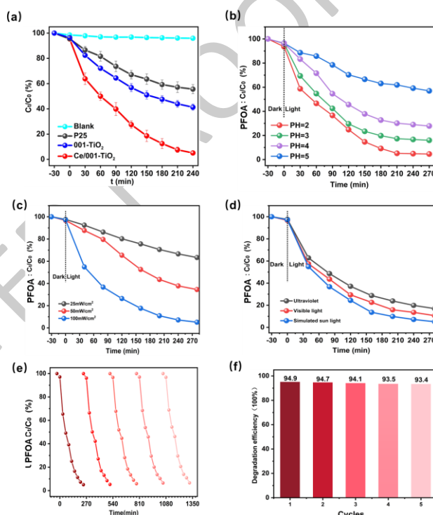
Figure 4. (a) Photocatalytic degradation curves of PFOA by P25, 001-TiO 2 , and Ce/001-TiO 2 , (b) Photocatalytic degradation curves of PFOA by Ce/001-TiO 2 under different pH values, (c) Photocatalytic degradation curves of PFOA by Ce/001-TiO 2 under varying light intensities, (d) Photocatalytic degradation curves of PFOA by Ce/001-TiO 2 under different light sources, (e) Photocatalytic degradation curves of PFOA by Ce/001-TiO 2 over five consecutive cycles, (f) Bar chart depicting the photocatalytic degradation of PFOA by Ce/001-TiO 2 over five cycles.
