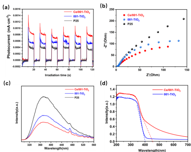
Figure 3. (a) Transient photocurrent response plots (I-t curves), (b) Electrochemical impedance spectra, (c) Steady-state photoluminescence (PL) spectra, (d) Ultraviolet-visible diffuse reflectance spectroscopy (UV-Vis DRS)
