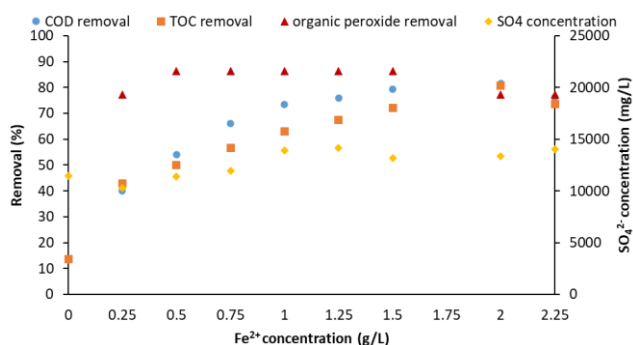
Figure 2. COD, TOC and organic peroxide removal efficiency at different \text{Fe}^{2+} concentrations ( \text{H}_2\text{O}_2 : 17.5 g/L, t: 60 min, pH: 3)
