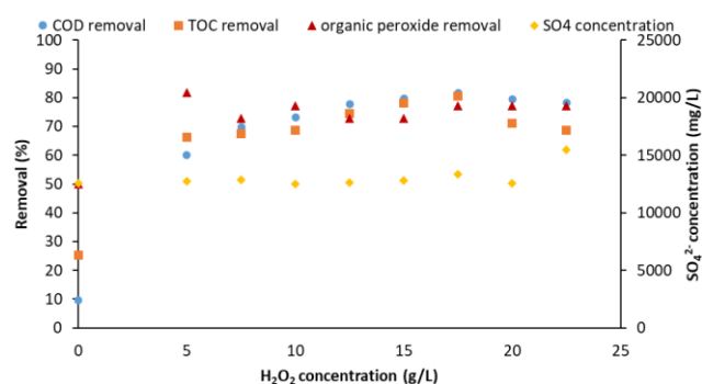
Figure 1. COD, TOC and organic peroxide removal efficiency at different \text{H}_2\text{O}_2 concentrations ( \text{Fe}^{2+} : 2.0 g/L, t: 60 min, pH: 3)
