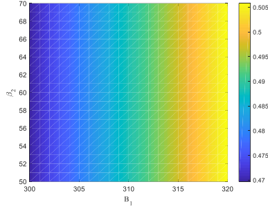
Figure 7. The threshold changes under the simultaneous influence of B_1 and \beta_2
