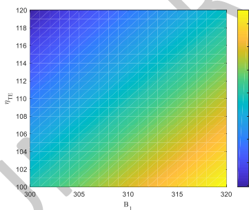
Figure 9. The threshold changes under the simultaneous influence of B_1 and \eta_{TE}
