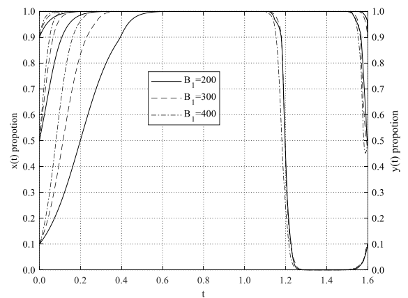
Figure 3. Impact of B_1 on system evolution
