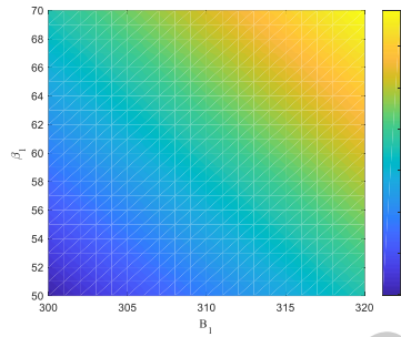
Figure 8. The threshold changes under the simultaneous influence of B_1 and \beta_1
