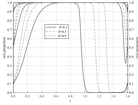
Figure 6. Impact of \theta on system evolution
