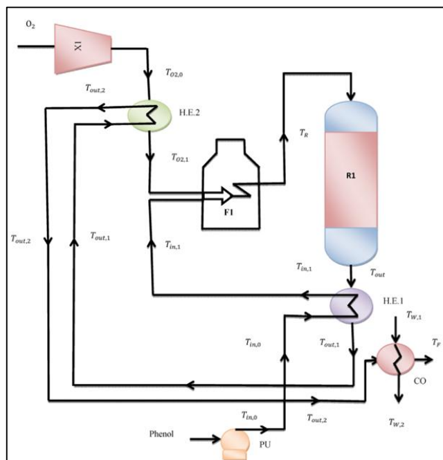
Figure 15. Schematic representation and energy saving of the process (Mohammed et al. 2017).
