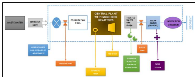
Figure 13. Process Flow Diagram of Variant V3 (Četković et al. 2022).
