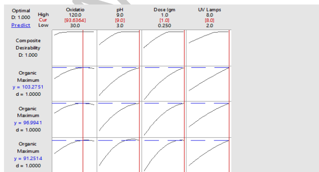
Figure 11. Finest independent variables with organic removal
