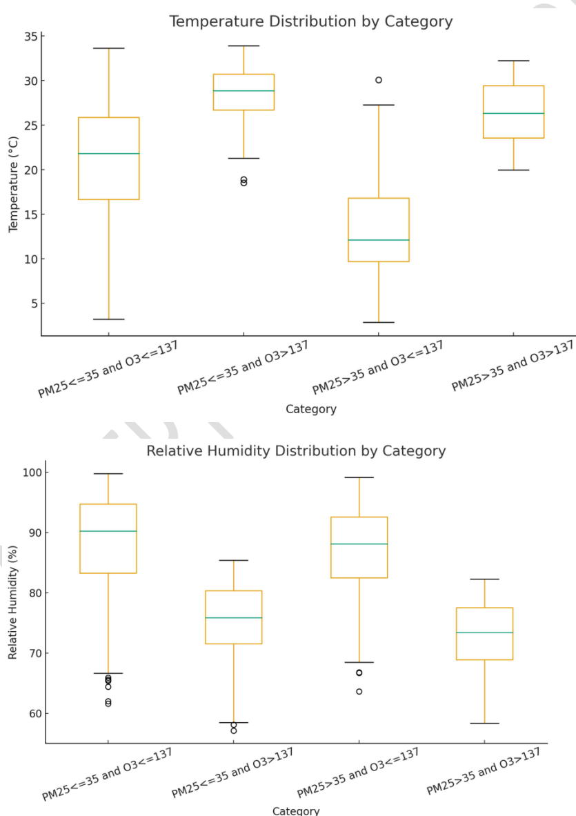
Figure 3. Distribution of temperature and relative humidity at the different \text{PM}_{2.5} and O_3
