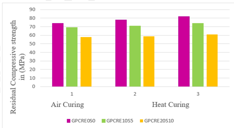
Figure 7: Residual Compressive strength of HSGPC mixes with 0,5 and 10% sulphate concentrations.
