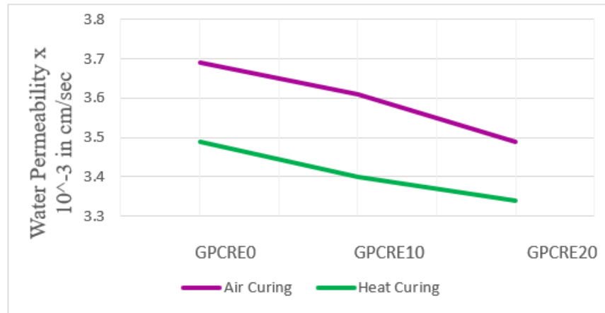
Figure 6: Water Sorptivity coefficient of HSGPC mixes.
