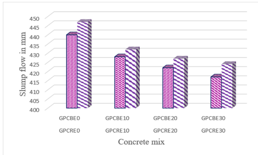
Figure 1: Slump Flow for different mixes of GPC
