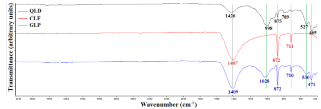
Figure 4. Fourier-transform infrared (FTIR) spectra of the limestone fillers
