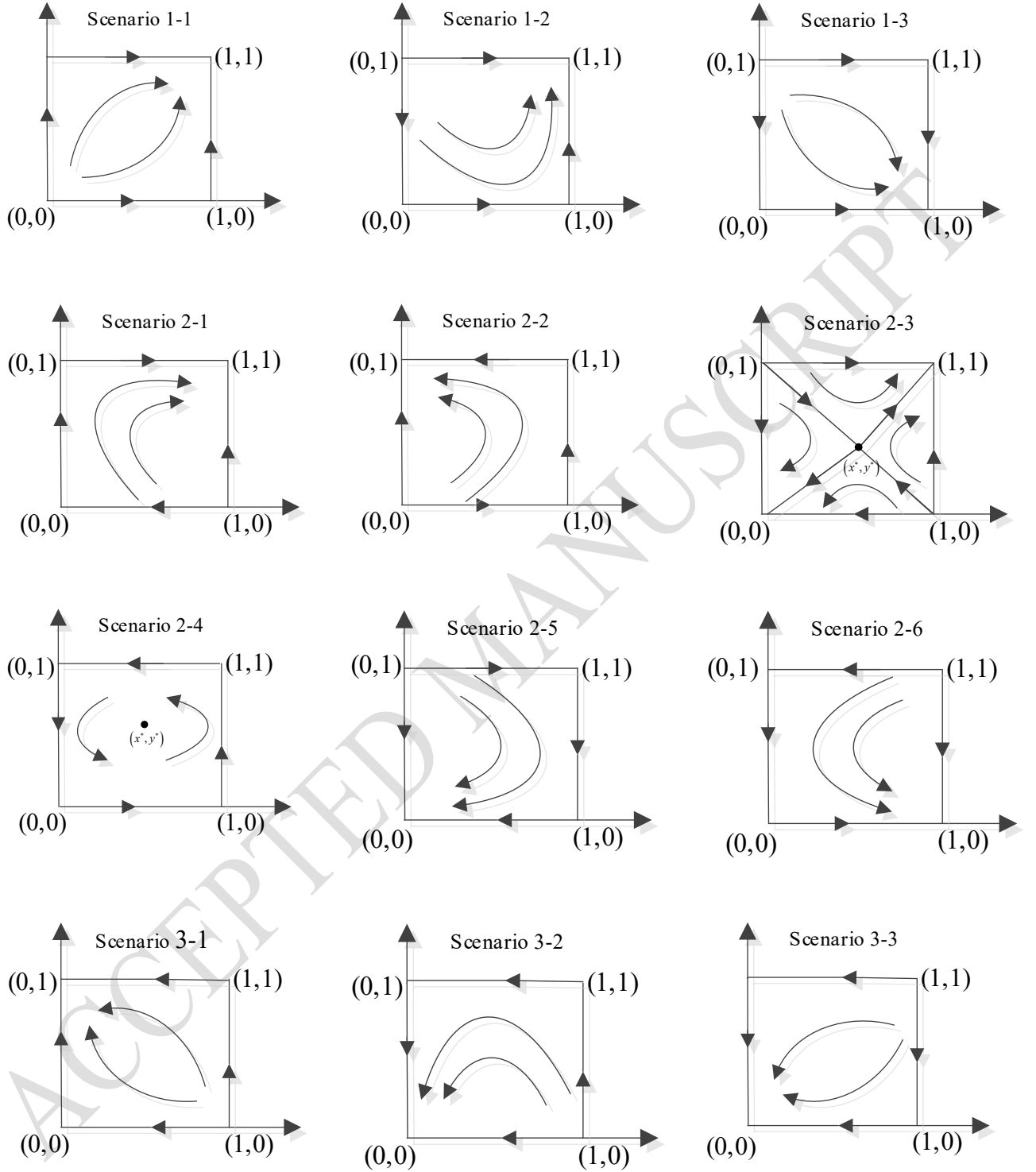
Figure 2 phase diagram of system evolution in scenarios 1-1 to 3-3
