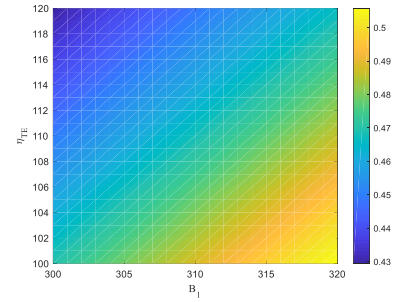
Figure 9 The threshold changes under the simultaneous influence of B_1 and \eta_{TE} .
