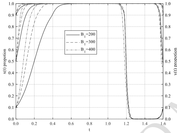
Figure 3 Impact of B_1 on system evolution
