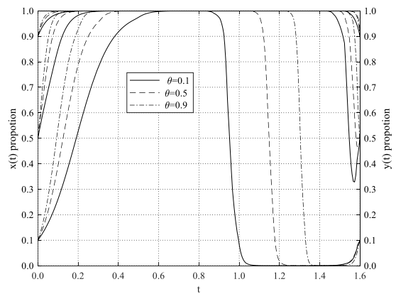
Figure 6 Impact of \theta on system evolution
