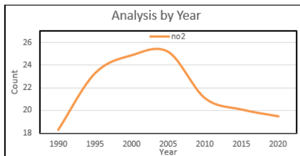
Figure-10. \text{NO}_2 measure for different years
