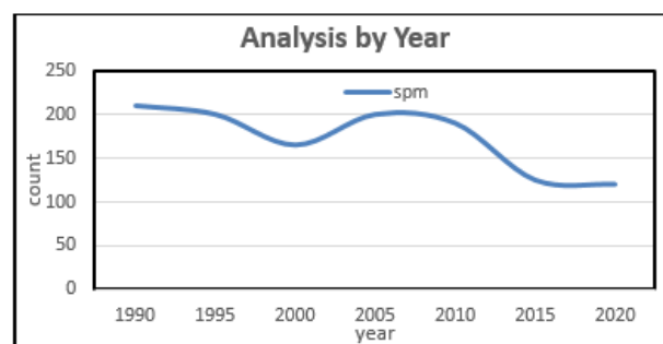
Figure-12. SPM Measure On Different Years
