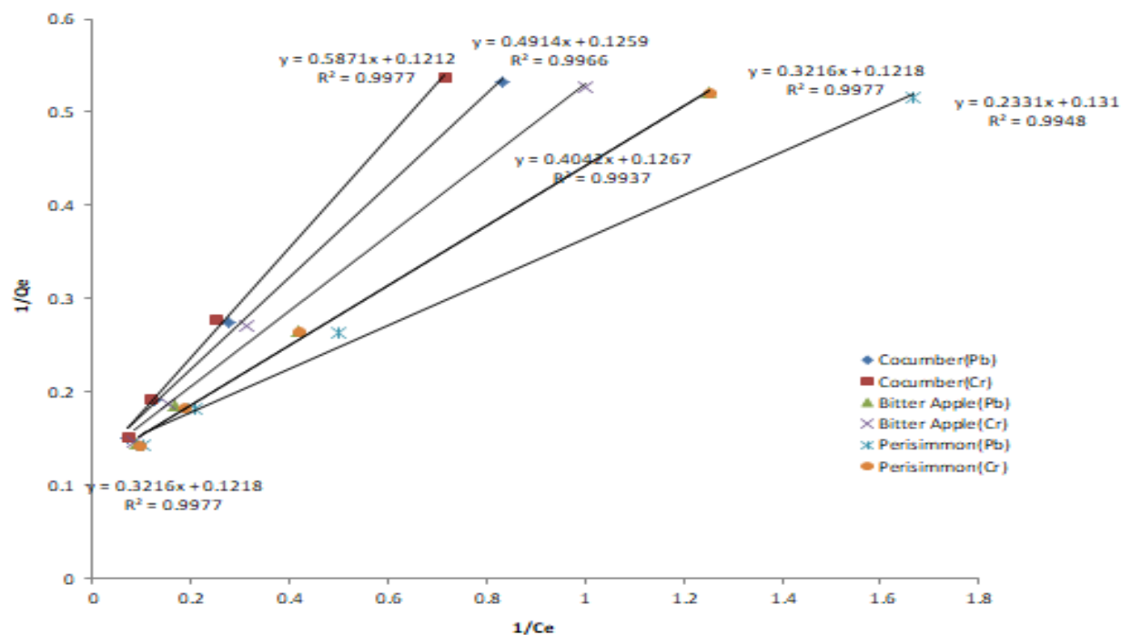
Figure 10. Langmuir Isotherm at Piplan
