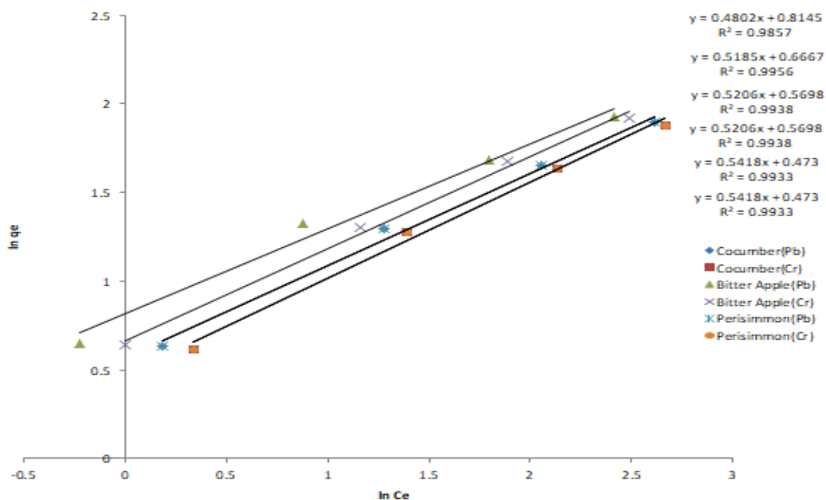
Figure 8. Freundlich Isotherm at Piplan
