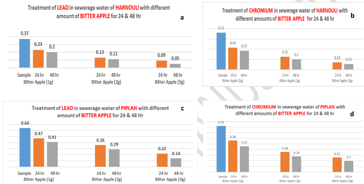
Figure 5: Effect of treatment of a) Pb in sewage water of Harnoli by different amounts of bitter apple, b) Cr in sewage water of Harnoli by different amounts of bitter apple, c) Pb in sewage water of Piplan by different amounts of bitter apple, d) Cr in sewage water of Piplan by different amounts of bitter apple
