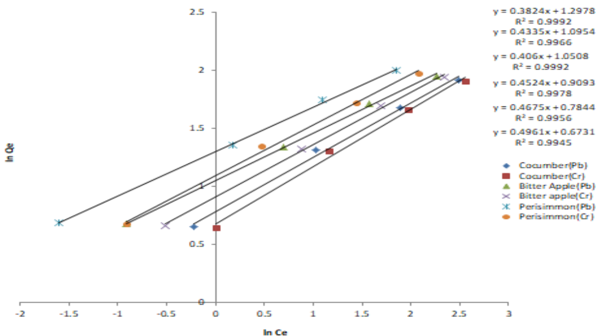
344 345 Figure 7. Freundlich isotherm at Harnouli 346
