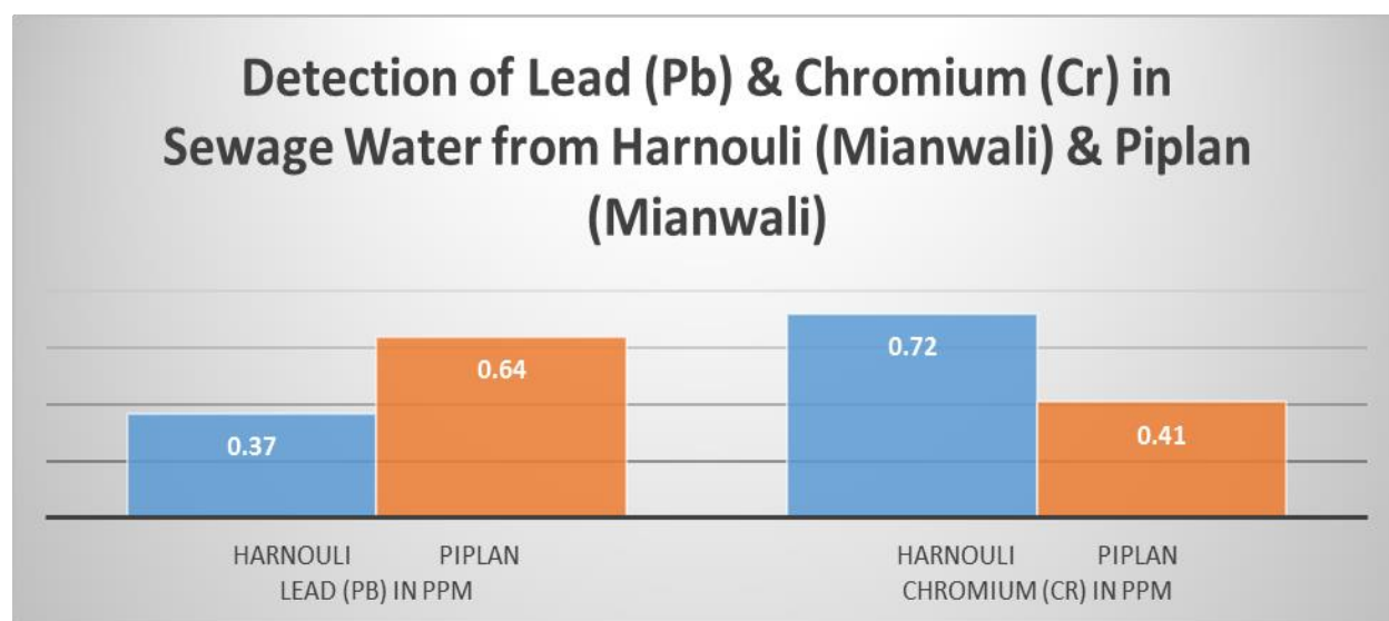
Figure 3. Detection of Pb and Cr in sewage water from Harnouil and Piplan
