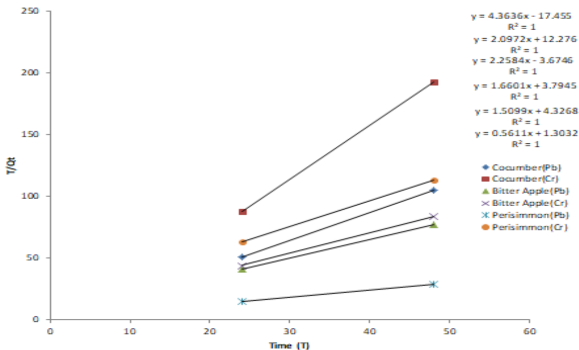
Figure 13. Pseudo-second-order kinetics at Harnouli
