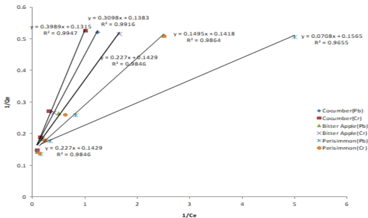
Figure 9. Langmuir Isotherm at Harnouli
