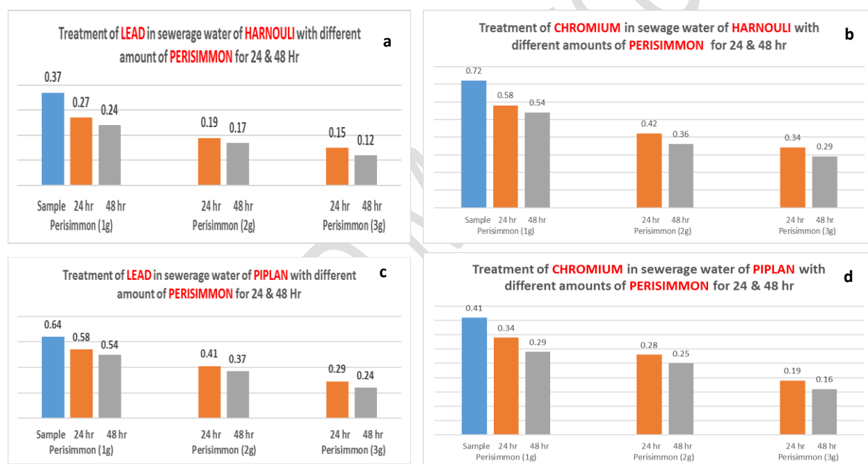
Figure 4: Effect of treatment of a) Pb in sewage water of Harnoli by different amounts of persimmon, b) Cr in sewage water of Harnoli by different amounts of persimmon, c) Pb in sewage water of Piplan by different amounts of persimmon, d) Cr in sewage water of Piplan by different amounts of persimmon
