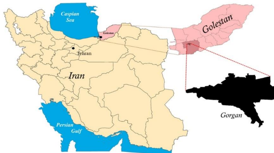
Figure 1. The location of the Gorgan Plain study area
