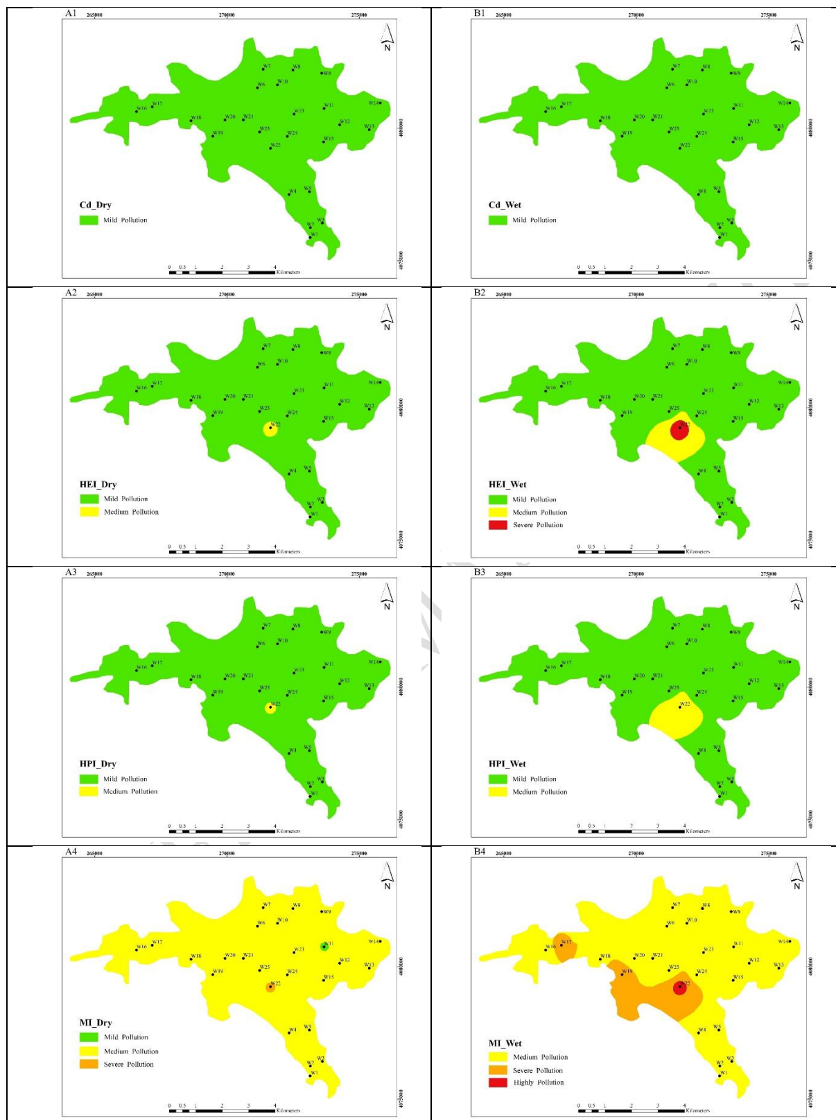
Figure 3. Classification of MI, HPI, HEI and pollution degree index (Cd) in (A) dry season and (B) wet season
