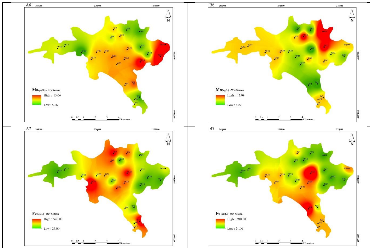
Figure 2. Spatial distributions of pollutants during wet and dry season samples
