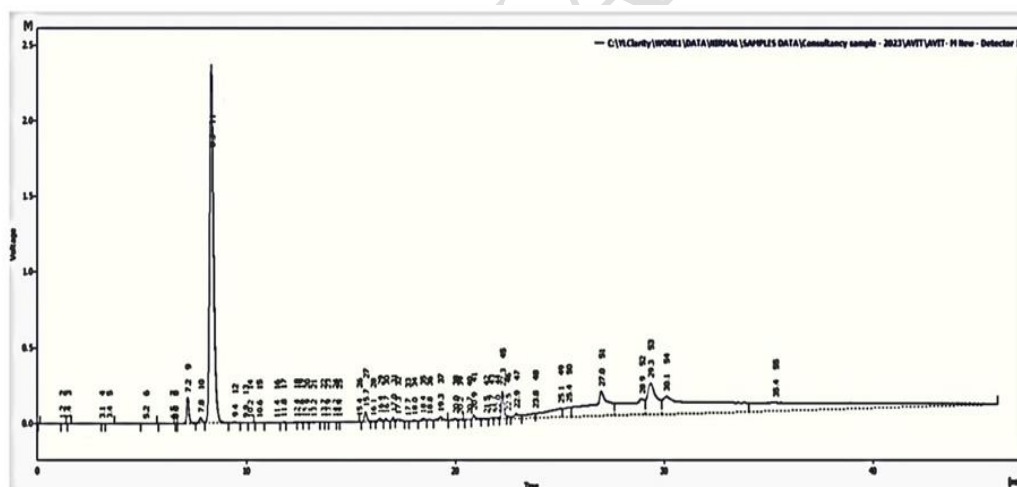
Fig: 5.GC-MS- Spectrum of Water extract of plants
