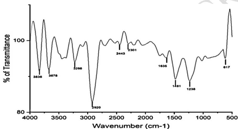
Fig 6. FTIR spectrum of hexane extracts
