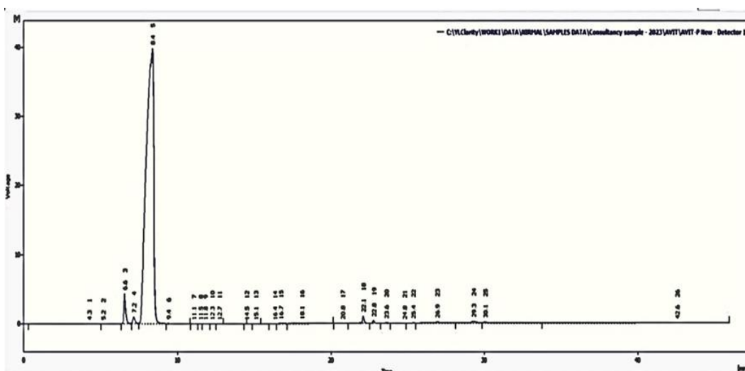
Fig: 4.GC-MS- Spectrum of Petroleum ether extract of plants
