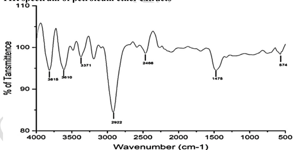
Fig -7: FTIR Spectrum of Petroleum ether extracts
