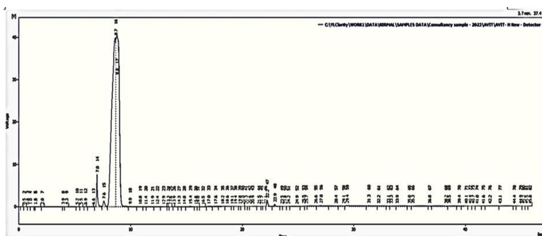
Fig: 3- GC-MS- Spectrum of Hexane extract of plants
