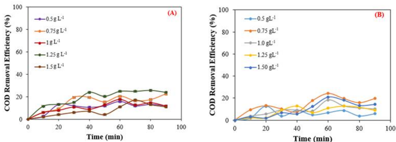
Figure 2. Effect of Fe^{2+} dosage on COD removal efficiency in the (a)Fenton and (b) photo-Fenton processes
