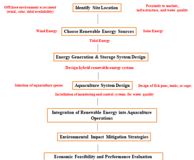
Figure 1. A flowchart for the design process of an integrated aquaculture system with aquaculture operations.
