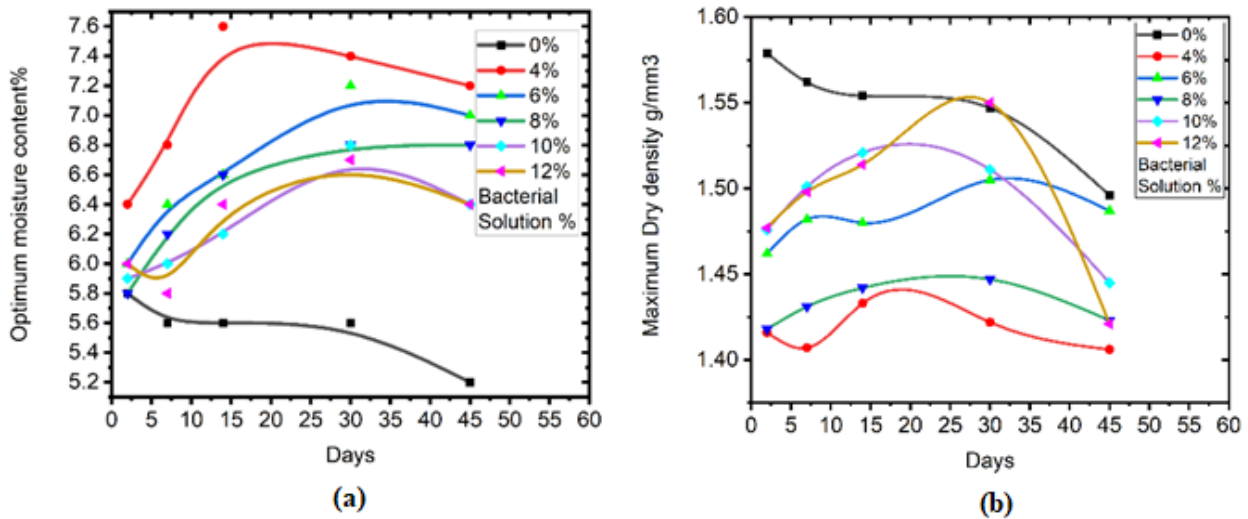
Fig 12: Biotreated sand Relationship between optimum moisture content and days for various percentage of bacterial solution added to 10% oil content soil sample.
