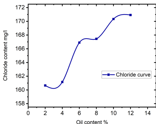
Fig 23: Oil contaminated sand relationship between chloride and oil content in 30 days curing period
