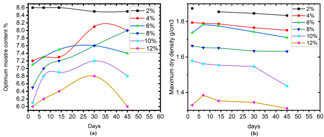
Fig 7: Oil contaminated sand : Relationship between optimum moisture content, maximum dry density and days for adding various percentage of oil in soil sample
