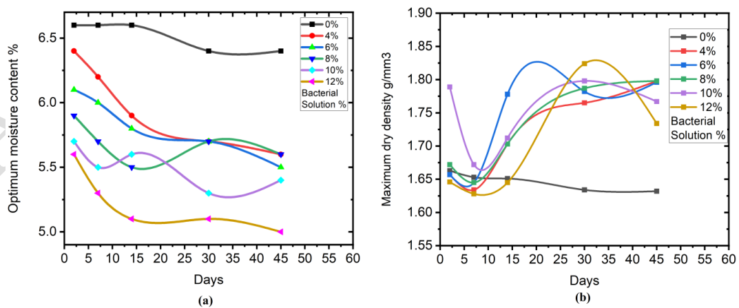
Fig 11: Bio treated sand: Relationship between optimum moisture content, maximum dry density and days for various percentage of bacterial solution added to 8% oil content soil sample
