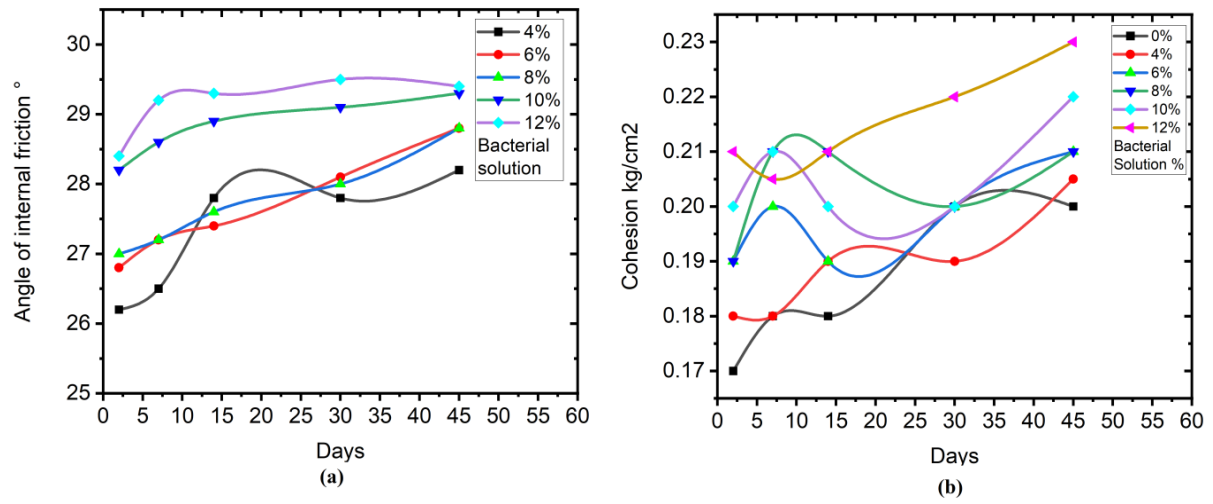
Fig 17 : Biotreated sand Relationship between Angle of friction , cohesion and days for various percentage of bacterial solution added to 6% oil content soil sample
