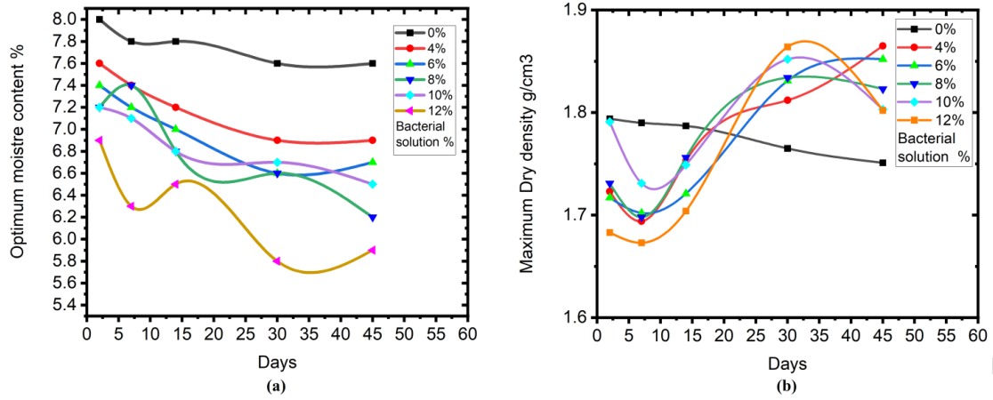
Fig 9: Biotreated sand: Relationship between optimum moisture content , maximum dry density and days for various percentage of bacterial solution added to 4% oil content soil sample
