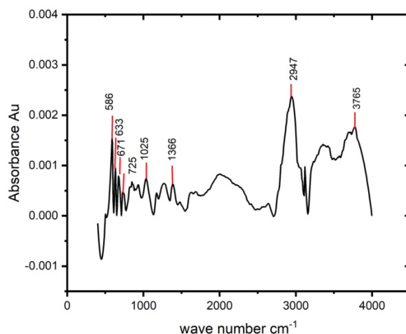
Fig 27: FTIR spectrum of 10% crude oil contaminated soil treated with 10 % bacterial solution after 30 days curing period
