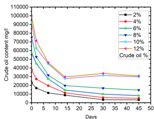
Fig 26: Biotreated sand: crude oil concentration of various oil percentage for different biotreatment time at 10% bacterial solution.
