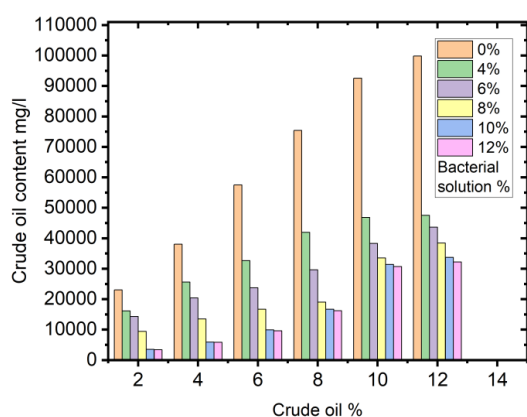
Fig 25: Biotreated sand: crude oil concentration of various bacterial concentration for various oil percentage at 30 days biotreatment time solution.
