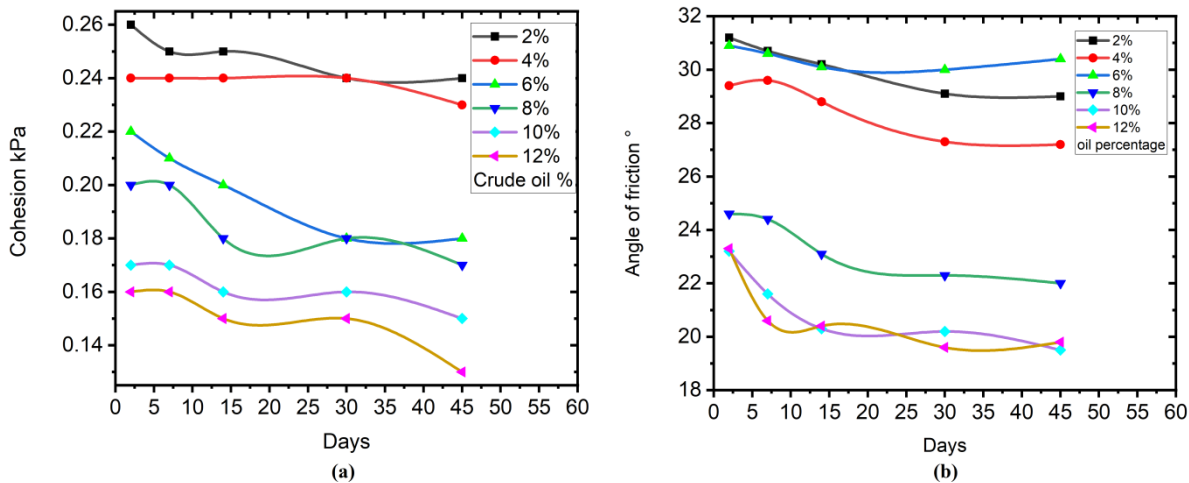
Fig 14: Oil contaminated sand: Relationship between Cohesion , Angle of friction and days for adding various percentage of oil in soil sample
