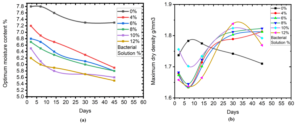
Fig 10 : Biotreated sand : Relationship between optimum moisture content, maximum dry density and days for various percentage of bacterial solution added to 6% oil content soil sample
