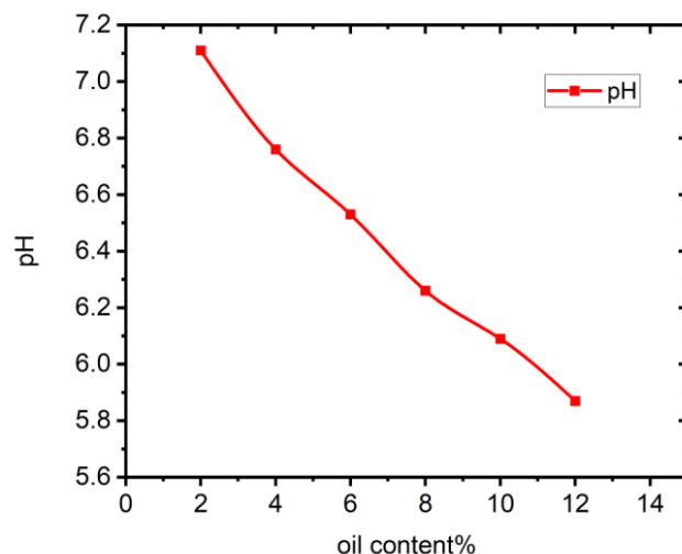
Fig 21: Oil contaminated sand: Relationship between ph and oil content 30 days curing period
