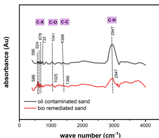
Fig 28: Comparative graph of FTIR spectrum of oil contaminated and biotreated sand
