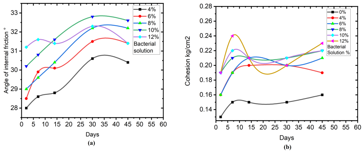
Fig 15: Biotreated sand Relationship between Angle of friction, cohesion and days, for various percentage of bacterial solution added to 2% oil content soil sample
