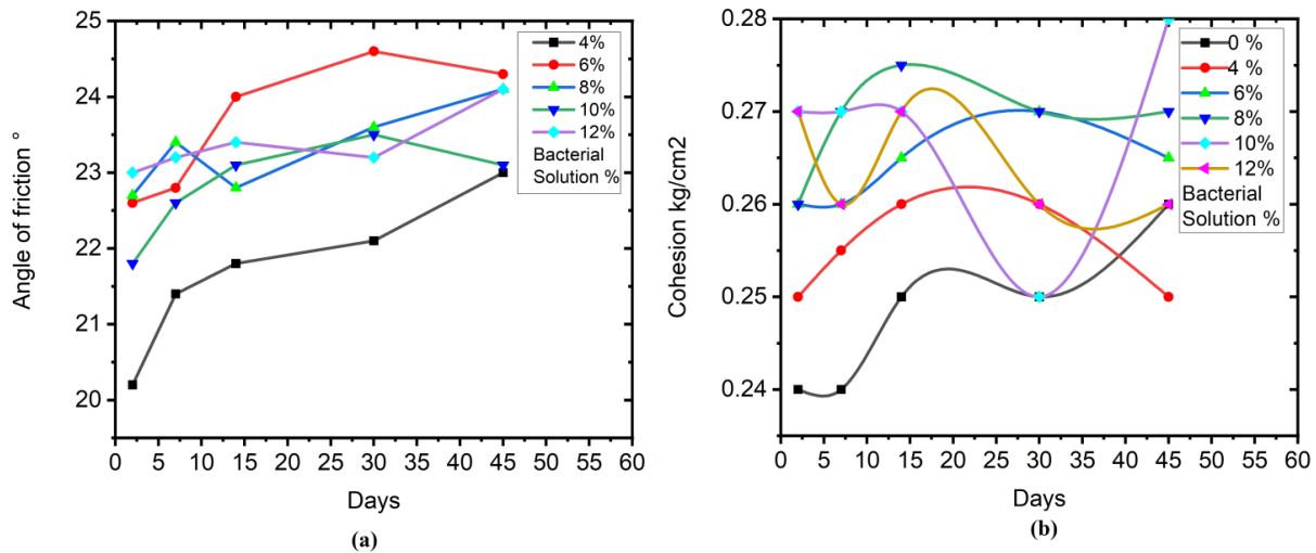
Fig 20: Biotreated sand: Relationship between Cohesion, Angle of friction and days for various percentage of bacterial solution added to 12% oil content soil sample.
