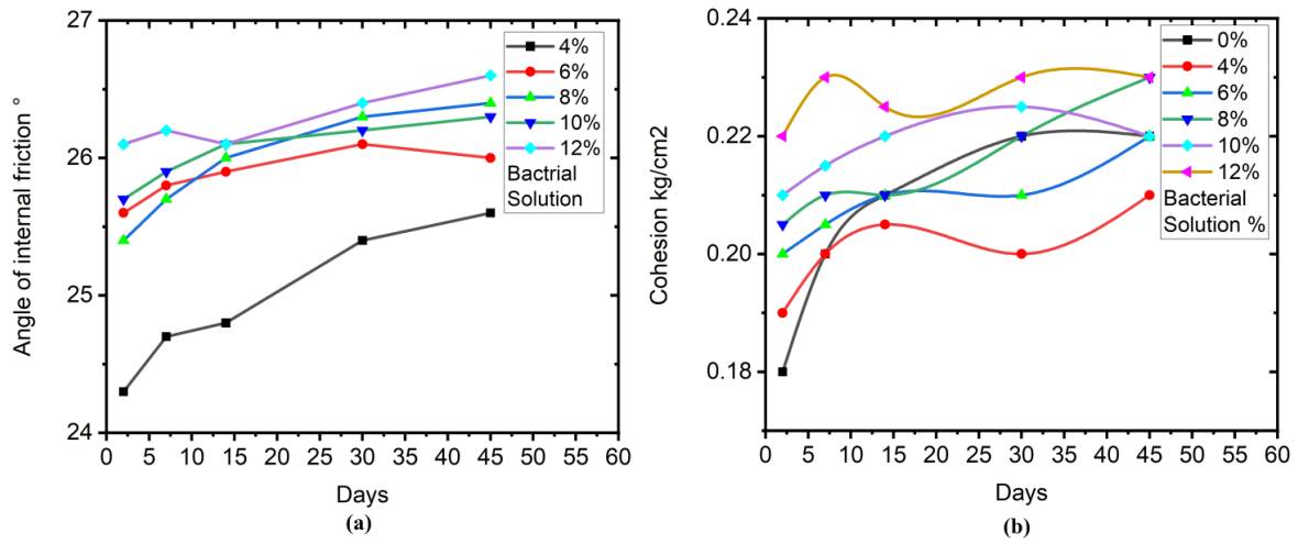
Fig 18 : Bio treated sand Relationship between Cohesion , Angle of friction and days for various percentage of bacterial solution added to 8% oil content soil sample
