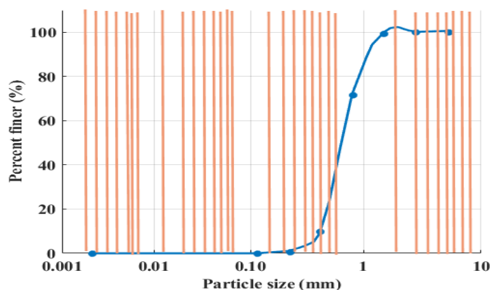
Fig 1: Particle size distribution curve of Marine sand
