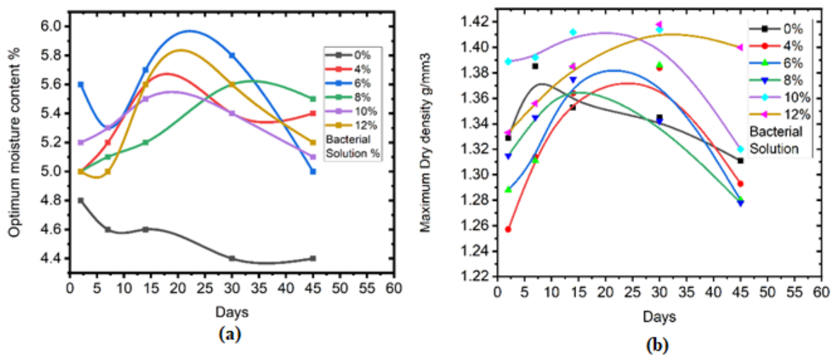
Fig 13 Biotreated sand Relationship between optimum moisture content ,maximum dry density and days for various percentage of bacterial solution added to 12% oil content soil sample.
