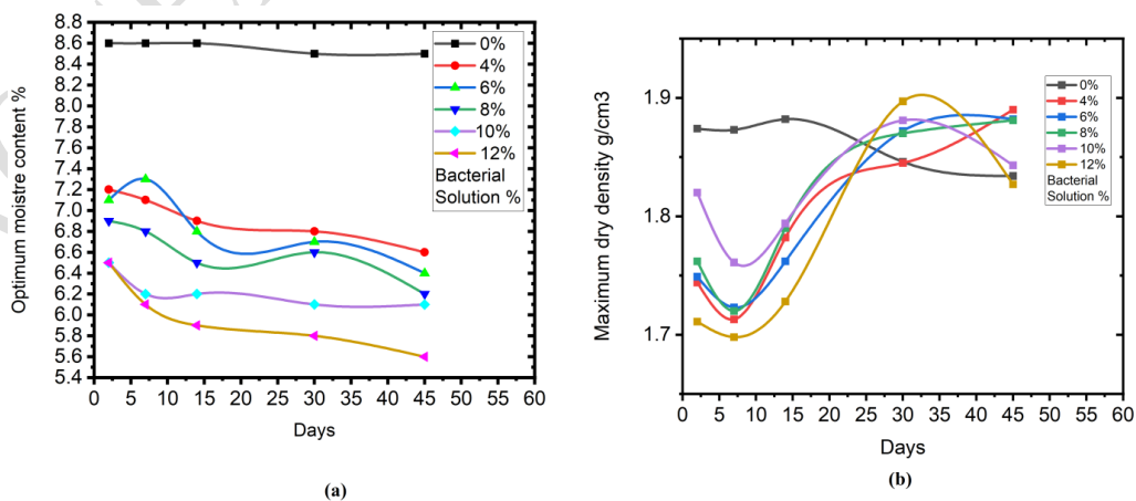
Fig 8: Biotreated sand: Relationship between optimum moisture content and days, maximum dry density and days for various percentage of bacterial solution added to 2% oil content soil sample
