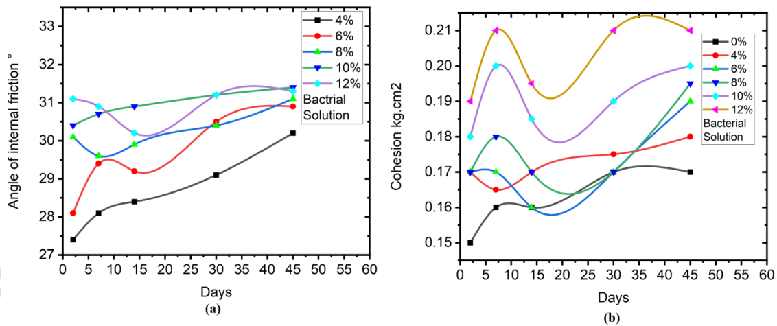
Fig 16: Bio treated sand Relationship between Cohesion, Angle of friction and days for various percentage of bacterial solution added to 4% oil content soil sample
