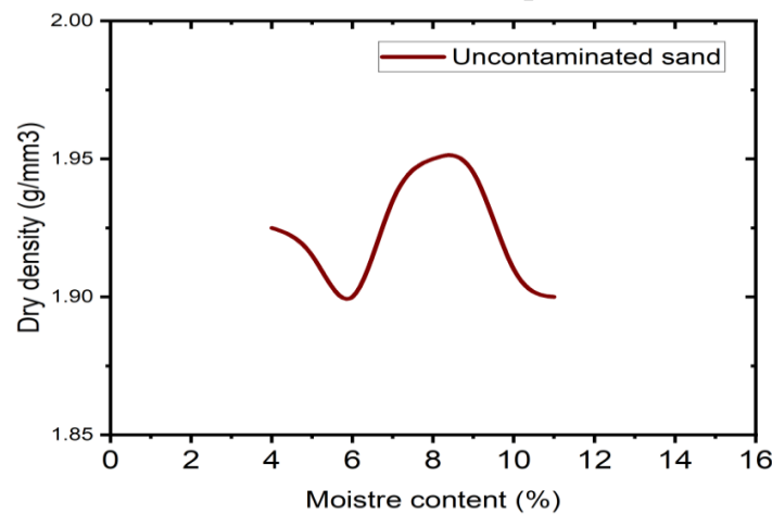
Fig 6: Compaction curve for uncontaminated sand
