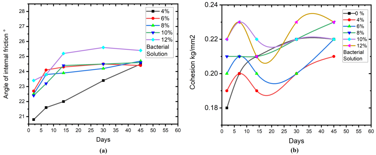
Fig 19 : Biotreated sand Relationship between Angle of friction , Cohesion for various percentage of bacterial solution added to 10% oil content soil sample
