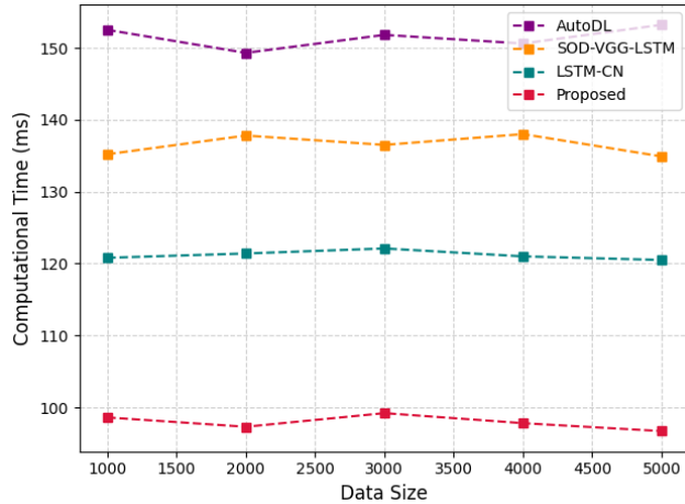
Figure 14. Comparison of Computational Time
