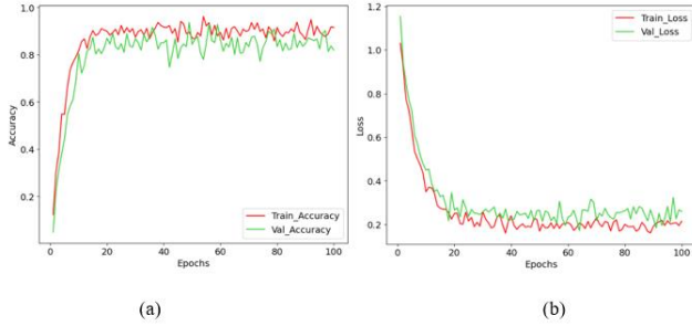
Figure 6. Accuracy and Loss curve for REWAR-Sense Method
