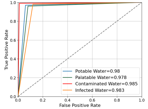
Figure 8. ROC Curve for REWAR-Sense Method
