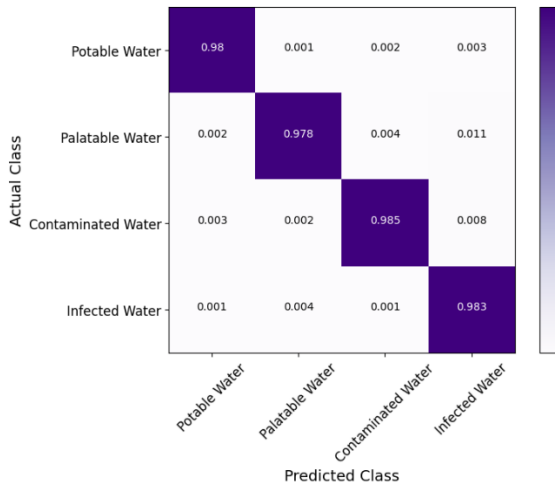
Figure 7. Confusion Matrix
