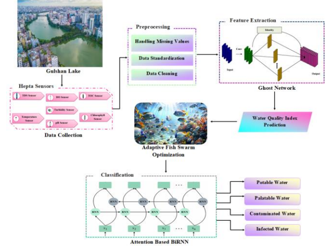
Figure 2. Proposed REWAR-Sense Methodology
