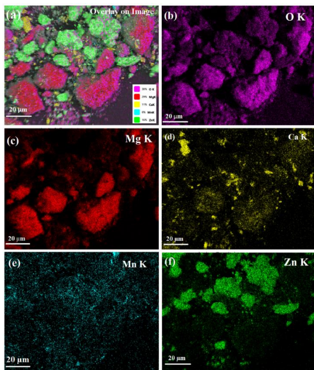
Figure 5. Elemental mapping for Mg-Zn-Ca-Mn nanocomposite
