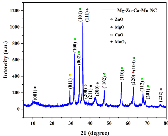
Figure 2. XRD analysis of the prepared Mg-Zn-Ca-Mn nanocomposite
