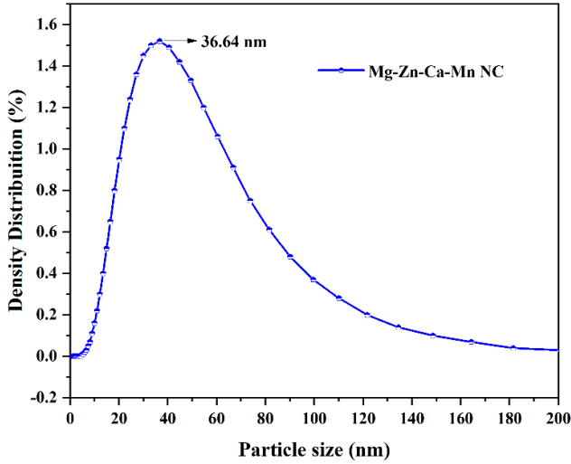
Figure 7. DLS analysis of prepared Mg-Zn-Ca-Mn nanocomposite. The d_{10} and d_{90} values of the prepared nanocomposite are 4.64 and 90.32 nm, respectively, indicating that the composite is present in the nanometre range. The broad peak observed in the result suggests that most of the particles in the prepared nanocomposite are available in a d_{50} range. The results also fit the previous SEM particle size and XRD crystalline size.
