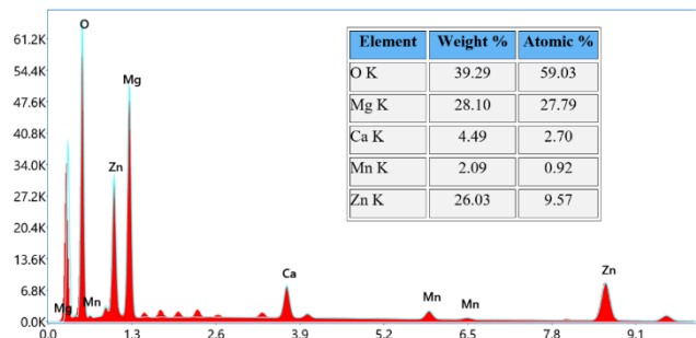
Figure 4. EDX spectrum of Mg-Zn-Ca-Mn nanocomposite
