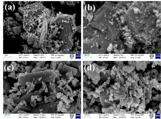
Figure 3. FESEM images of Mg-Zn-Ca-Mn nanocomposite
