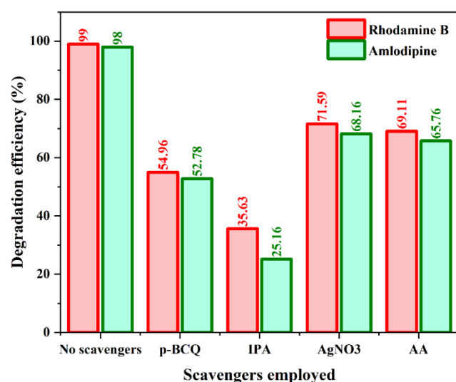
Figure 14. Evaluation of ROS responsible for the degradation of pollutants
