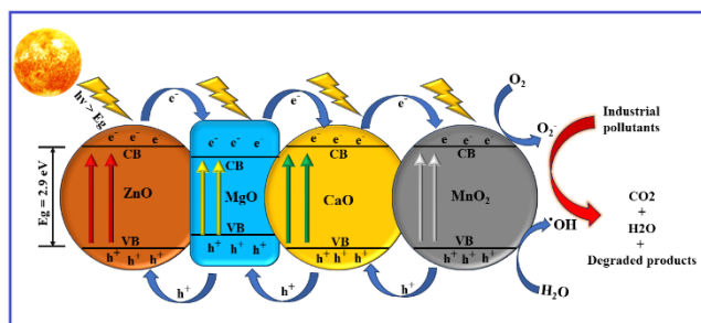
Figure 15. Photocatalytic degradation mechanism of Mg-Zn-Ca-Mn nanocomposite
