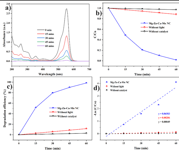
Figure 13. Photocatalytic performance on Rhodamine B: a) Time-dependent degradation, b) C/C_0 , c) degradation efficiency, and d) Pseudo first-order kinetics
