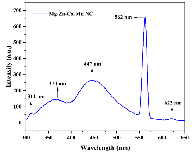
Figure 9. PL spectra of Mg-Zn-Ca-Mn nanocomposite
