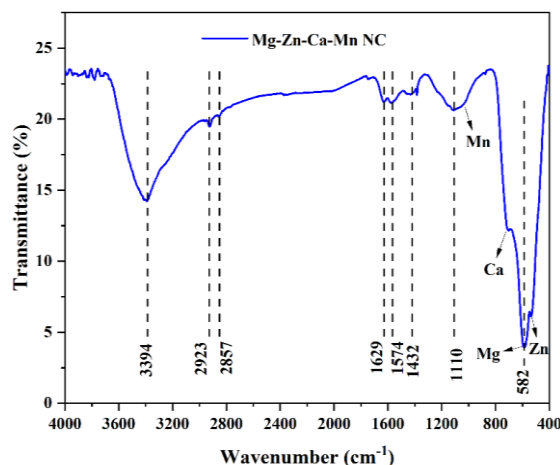
Figure 6. FTIR analysis of Mg-Zn-Ca-Mn nanocomposite
