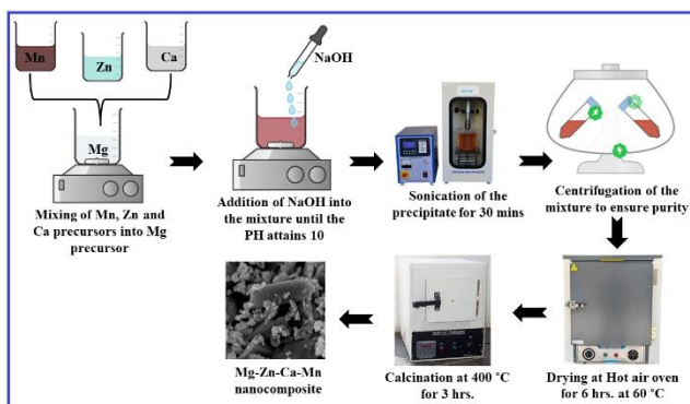
Figure 1. Preparation of Mg-Zn-Ca-Mn nanocomposite.
