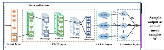
Figure 8. Shows the LSTM with convolution model handling n different samples.
