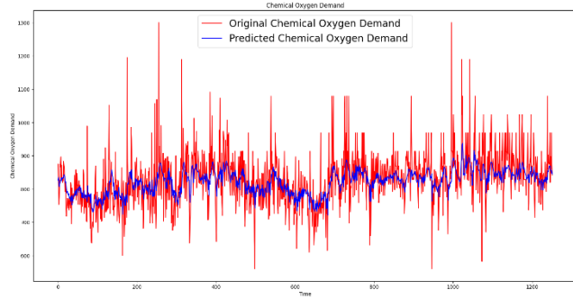
Figure 10b Actual Vs Predicted COD.
