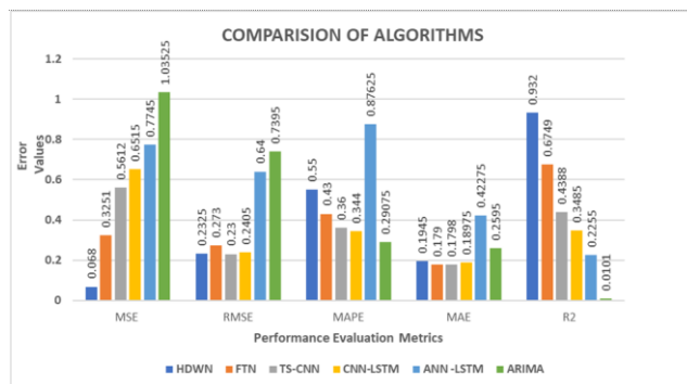
Figure 12. Comparison of Proposed Model Evaluation with other algorithms.
