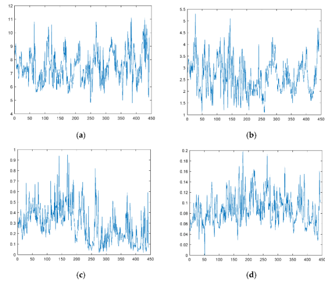
Figure 9. Sample Data set (a) Shows the pH level measured with the water sample (b) the COD of the water level (c) shows the BOD in water sample (d) The Total Nitrogen level in the water sample.
