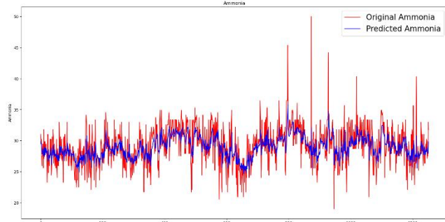
Figure 10c. Actual Vs Predicted Ammonia.
