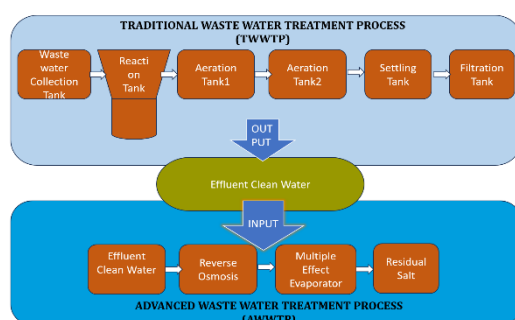
Figure 2 Waste Water Treatment Process.
