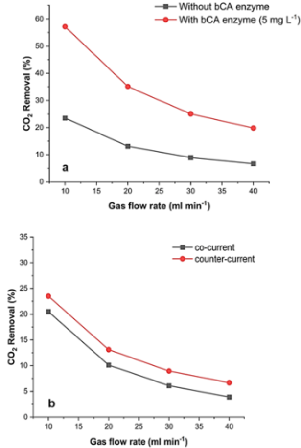
Figure 3. CO 2 removal as function of gas flow rate, C_{\text{CO}_2} = 5.24 \text{ mol m}^{-3} , bCA enzyme concentration = 5 mg L -1 , Q_l = 10 \text{ ml min}^{-1} , 0.5M (Na 2 CO 3 -NaHCO 3 ), T = 298 \text{ K} , \text{pH} = 9.6
