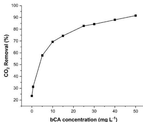
Figure 5. CO 2 removal as function of bCA enzyme concentration, C_{\text{CO}_2} = 5.24 mol m -3 , T = 298 K, pH= 9.6, Q_l = 10 ml min -1 , n=11 , Counter-current flow
