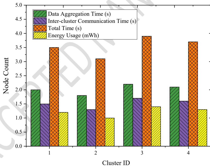
Figure 8. Clustering Performance in AQC-MANET
