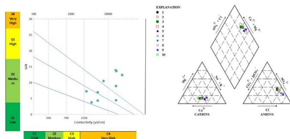
Fig. Classification of irrigation waters by USSL (after Richards 1954)
