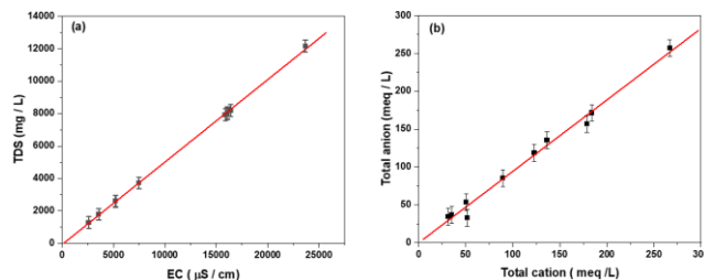
Figure 2. Correlation between TDS and EC (a); Total anion and cation (b)
