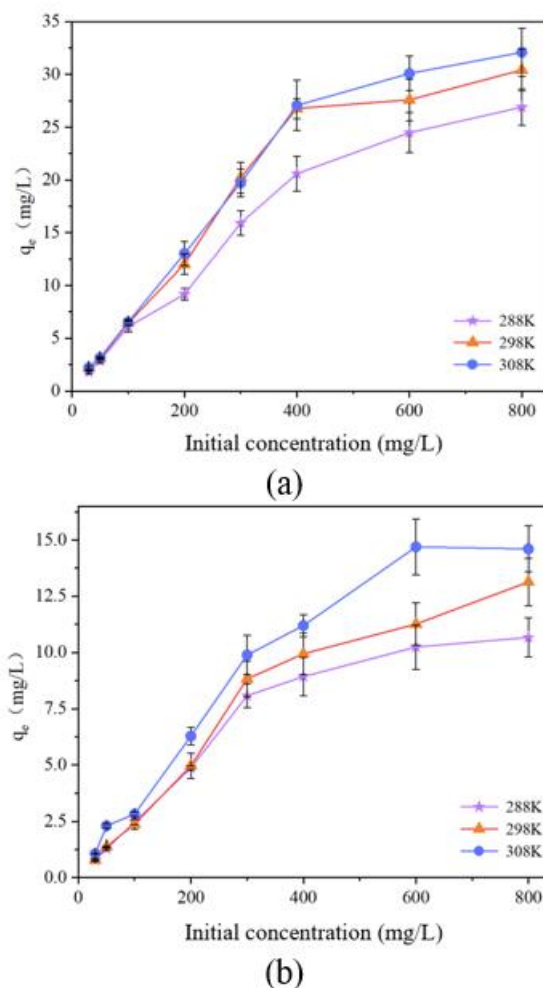
Figure 6. Effect of initial concentration and temperature on the adsorption of COD by high-temperature carbonizations: (a) Adsorption effect of SJC on COD; (b) Adsorption effect of SSC on COD
