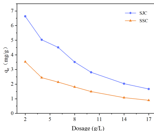
Figure 8. Effect of dosage on the adsorption of \text{NH}_4^+\text{-N} by high-temperature carbonization
