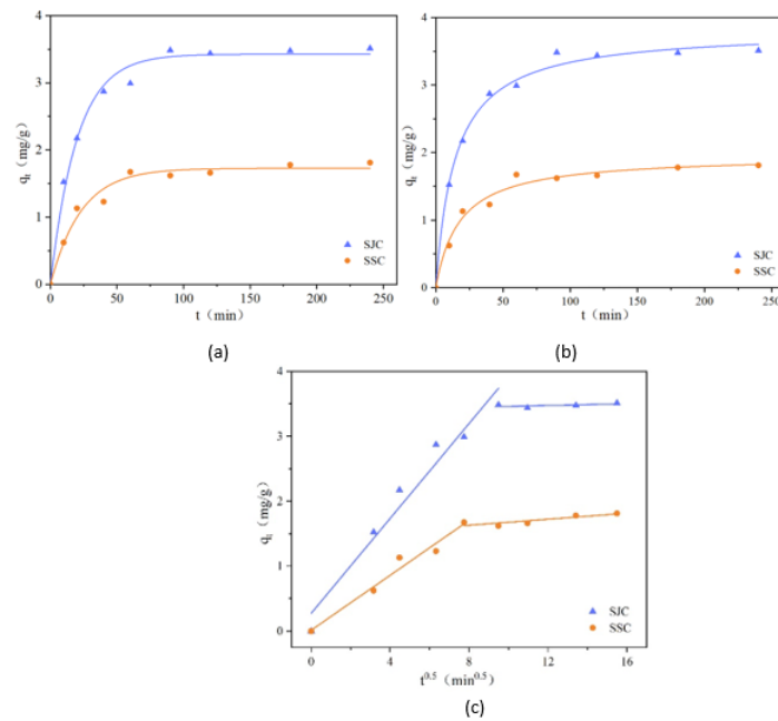
Figure 12. Fitting diagram of the kinetic model of adsorption of \text{NH}_4^+\text{-N} by SJC and SSC; (a) Pseudo-first order kinetic model; (b) Pseudo-second order kinetic model; (c) Intragranular diffusion model
