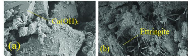
Figure 11. SEM image of (a) Control concrete (b) Effluent added concrete
