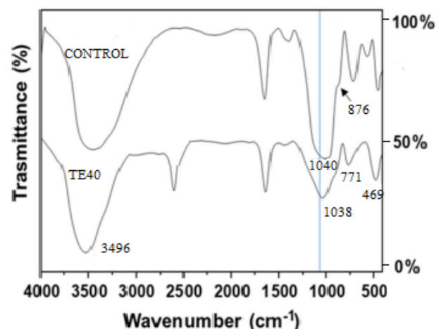
Figure 12. FT-IR spectra of control mix and mix TE40
