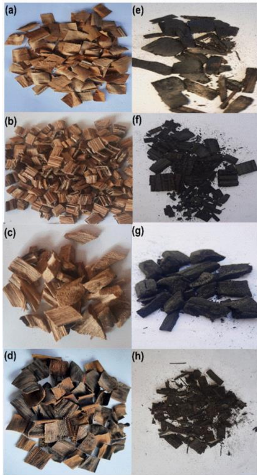
Figure 3. Plant parts and their corresponding biochar (a) leaves (b) pseudostem (c) peduncle (d) bud bract (e) leaves biochar (f) pseudostem biochar (g) peduncle biochar and (h) bud bract biochar
