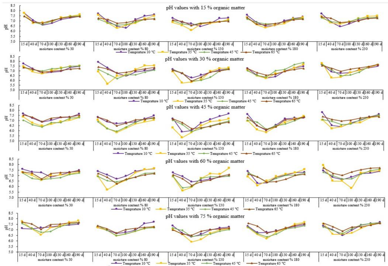
a. pH value changes w.r.t Organic Matter Content, Moisture Content and Temperature
