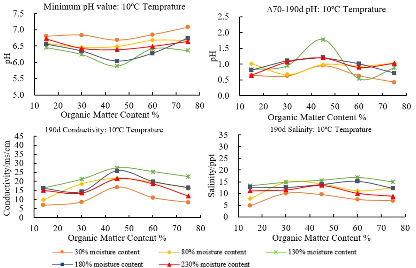
Figure 5. Effect of temperature on the degradation characteristics of MSW
