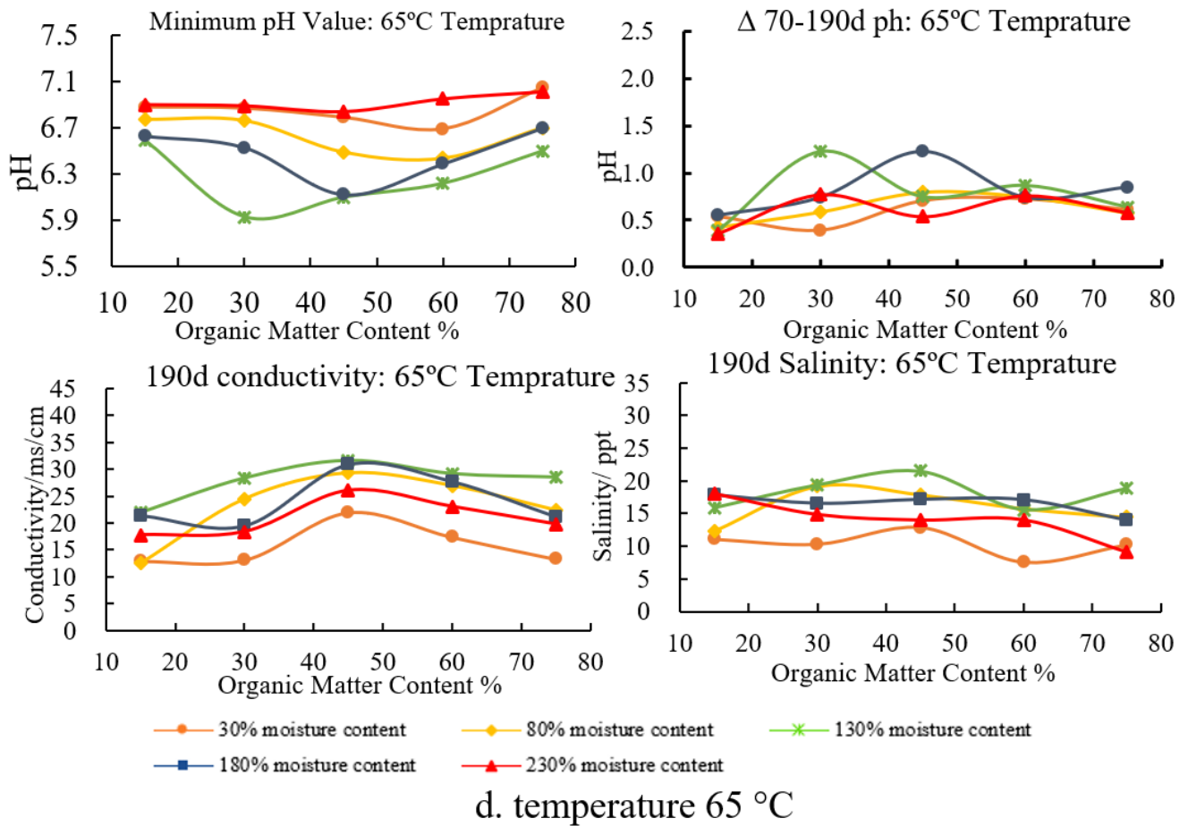
Figure 6. Effect of organic matter content on the degradation characteristics of MSW
