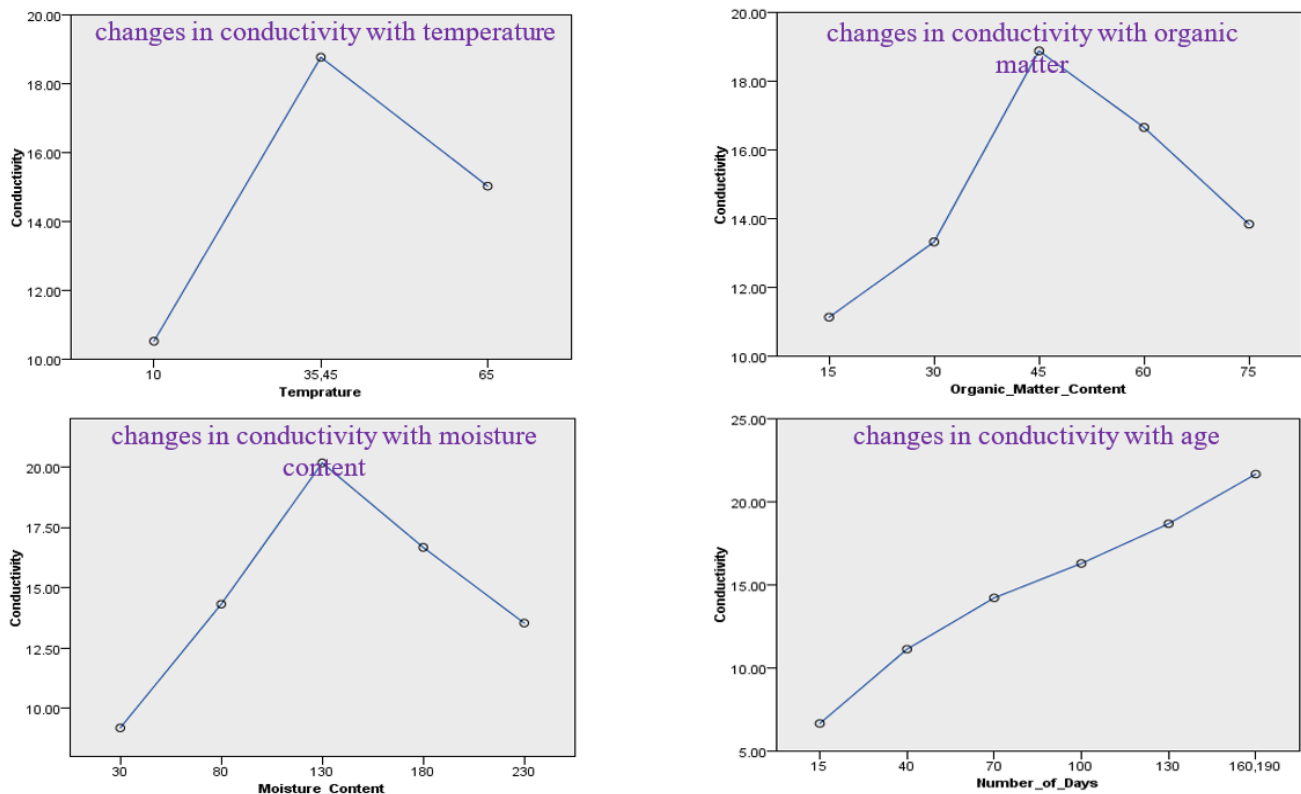
e. Estimated Mean Values (Conductivity)
