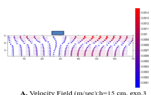
Figure 16. Results of mathematical model-velocity field h=15 cm exp.3
