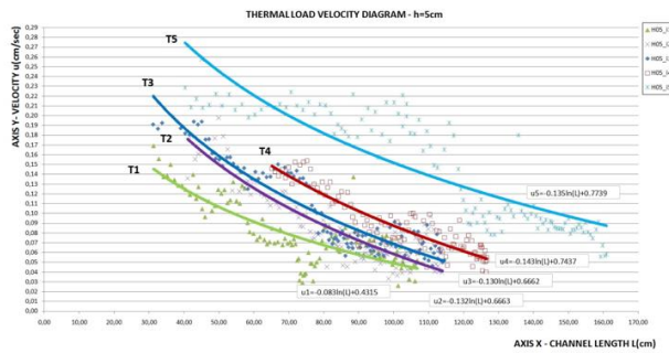
Figure 22. Experimental Mean velocity fields u (cm/sec) on the channel axis ( X ) for h = 5 cm
