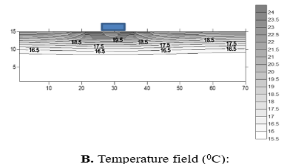
Figure 17. Results of a mathematical model - temperature field h=15 cm exp.3
