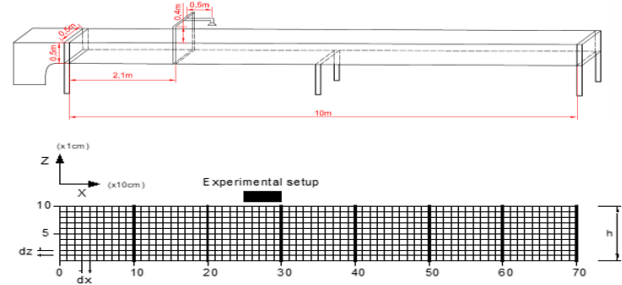
Figure 1. Schematic representation of calculation canvas generation with different length-height scales
