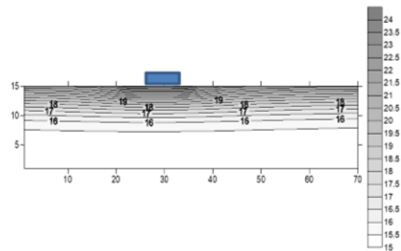
Figure 18. Results of mathematical model-velocity field h=15 cm exp.4
