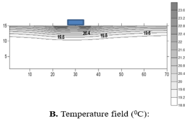
Figure 13. Results of a mathematical model - temperature field h=15 cm exp.1
