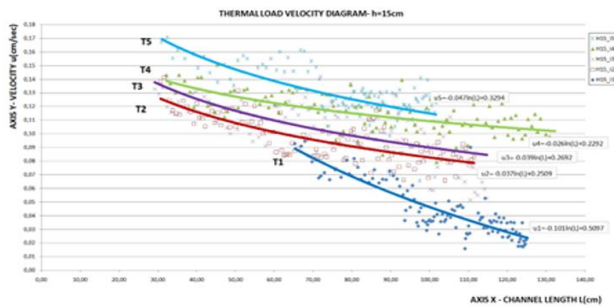
Figure 23. Experimental Mean velocity fields u (cm/sec) on the channel axis ( X ) for h = 15 cm
