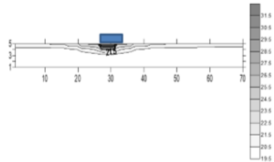
Figure 4. Results of mathematical model-velocity field h=5 cm exp.2
