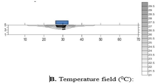
Figure 3. Results of the mathematical model-temperature field h=5cm exp.1
