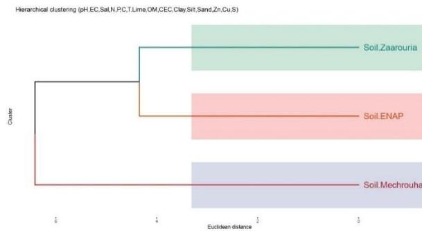
Figure 3. Hierarchical classification of sampling sites of C. aspersum (Zaarouria, Mechrouha and ENAP) based on soil physicochemical parameters and TME.
