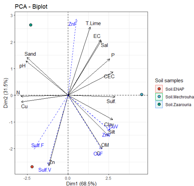
Figure 2. Principal component analysis (PCA) biplot of the three sampled site characterization (Dim 1: 68.5% and Dim 2 = 31.5%).
