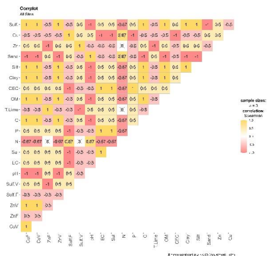
Figure 7. Spearman's correlation carried out on TME, sulfates and physicochemical parameters measured in both snails' tissues and soil samples in all sites.
