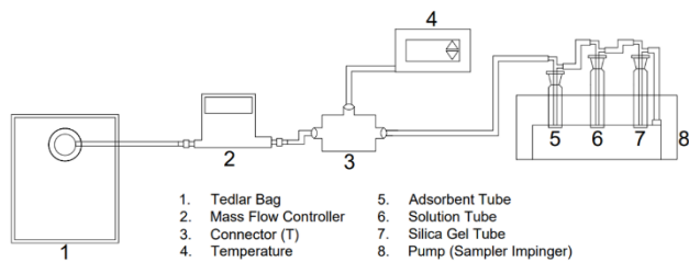
Figure 1. Simple Arranged Equipment
