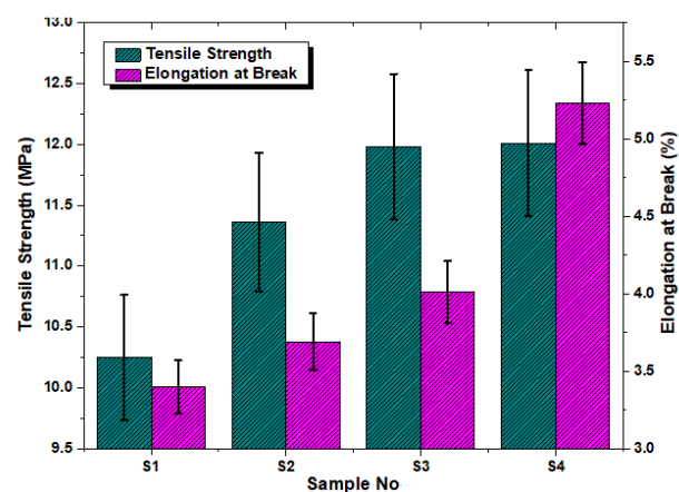
Figure 6. Mechanical Properties of Plain Chitosan Powder (S1) and chitosan and silver particles-based Hybrid composites (S2, S3 and S4)
