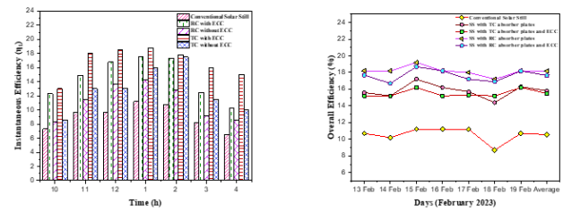
Figure 5. Evaluation of (a) instantaneous efficacy at variant hours a day, (b) total efficacy at variant testing days between variant solar stills
