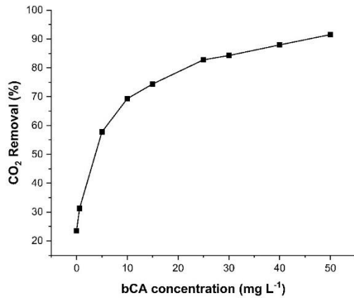
Figure 5. CO 2 removal as function of bCA enzyme concentration, C_{CO_2} = 5.24 mol m -3 , T = 298 K, pH = 9.6, Q_l = 10 ml min -1 , Q_g = 10 ml min -1 , n=11, Counter-current flow
