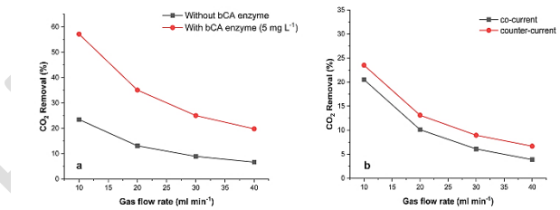
Figure 3. CO 2 removal as function of gas flow rate, C_{\text{CO}_2} = 5.24 \text{ mol m}^{-3} , bCA enzyme concentration = 5 mg L -1 , Q_l = 10 \text{ ml min}^{-1} , 0.5M (Na 2 CO 3 -NaHCO 3 ), T = 298 \text{ K} , \text{pH} = 9.6
