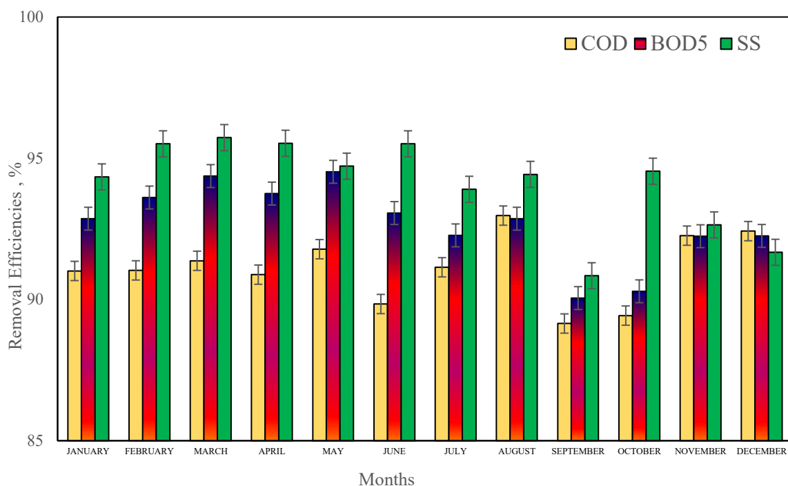
Figure 3. COD, BOD 5 , and SS (%) removal efficiencies
