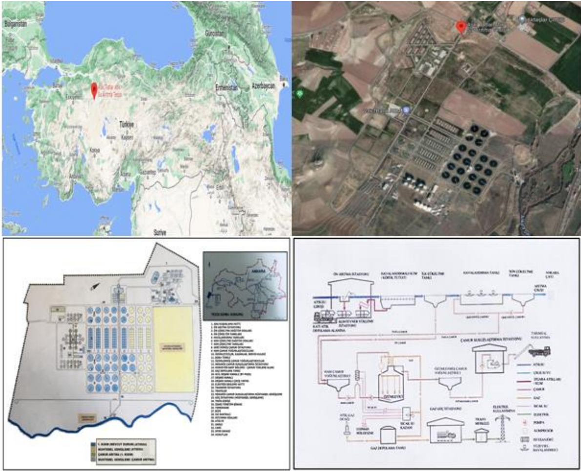
Figure 1. General layout and satellite image of Tatlar Wastewater Treatment Plant
