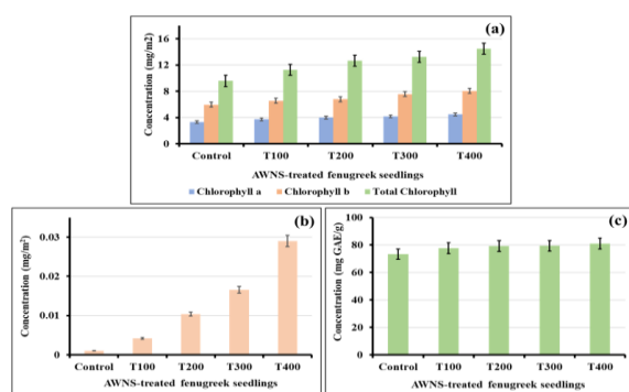
Figure 5. AWNS-treated fenugreek seedlings (a) Chlorophyll content, (b) Silica content, and (c) Polyphenol content
