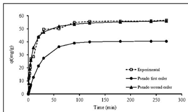
Figure 8. Predicted curve fits for the kinetics of methylene blue adsorption C_{0, BM}= 60 mg/L
