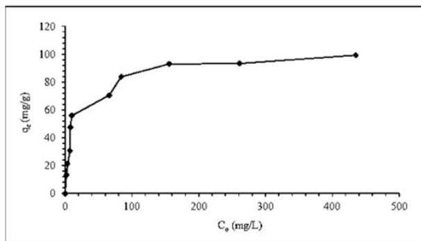
Figure 10. Isotherm of methylene blue adsorption
