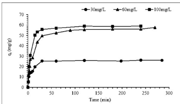
Figure 5. Effect of contact time and MB concentration on adsorption capacity onto
