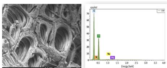
SEM image of NaOH-activated peanut shells
