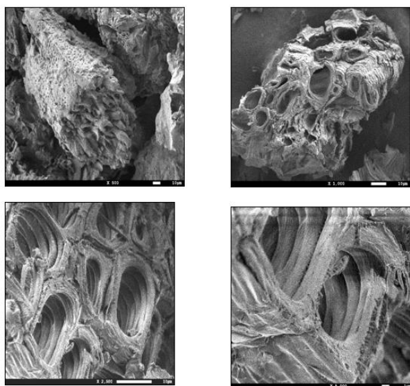
Figure 1. SEM image of NaOH-activated peanut shells
