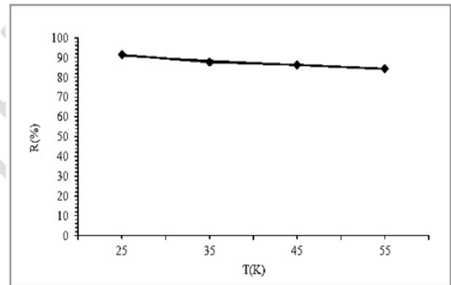
Figure 6. Effect of temperature on adsorption capacity of MB onto activated peanut shells
