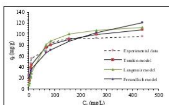
The predicted curve fits for equilibrium isotherms of methylene blue adsorption
