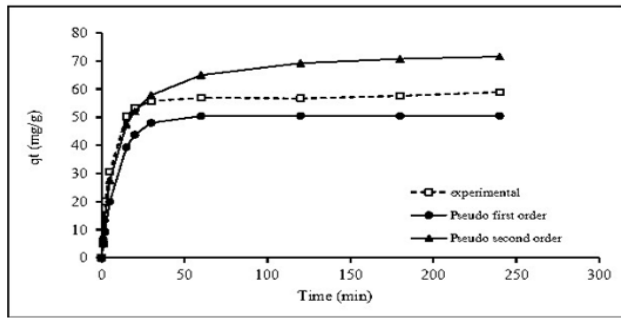
Figure 9. Predicted curve fits for the kinetics of methylene blue adsorption, C_0, BM=100 mg/L
